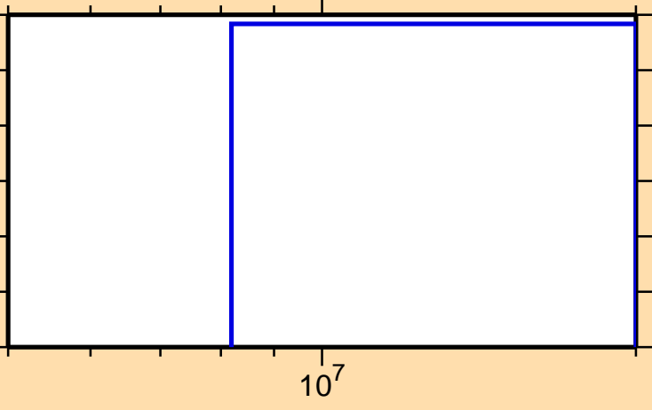
\sigma vs. E for ^{166}\text{Lu}(n,3n)
