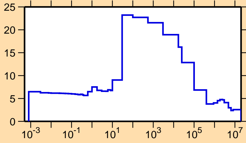
\sigma vs. E for ^{166}\text{Lu}(n,\text{el.})
