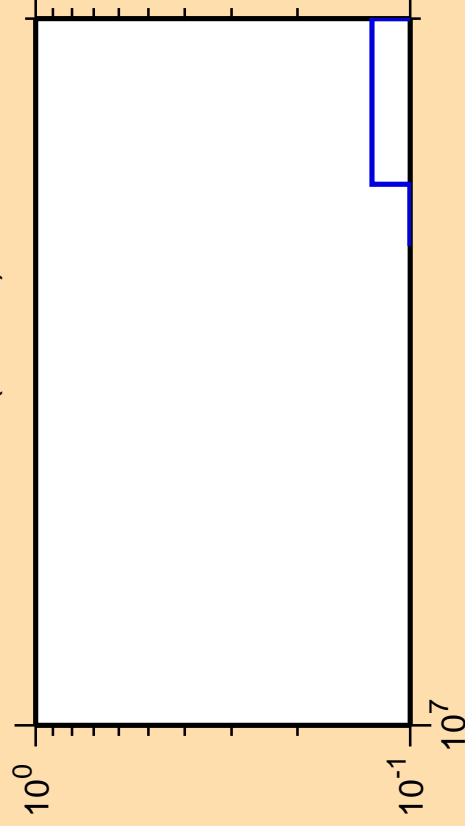
\Delta\sigma/\sigma vs. E for ^{166}\text{Lu}(n,3n\alpha)
