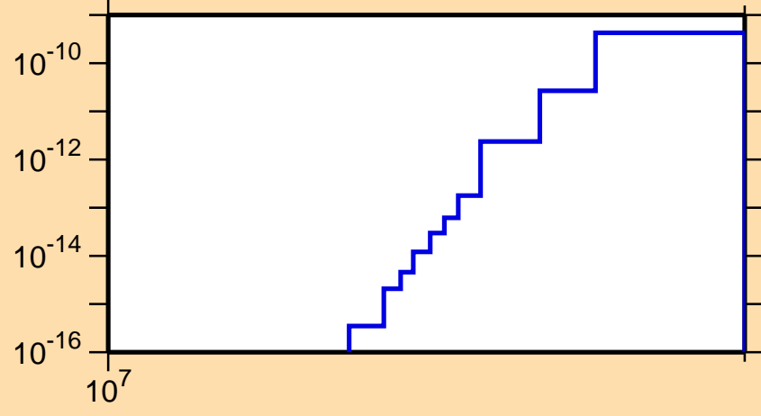
\sigma vs. E for ^{166}\text{Lu}(n,pd)
