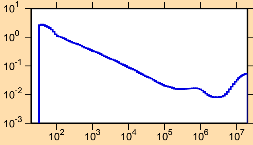
\sigma vs. E for ^{166}\text{Lu}(n,p)
