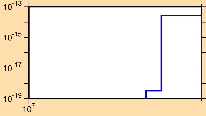
\sigma vs. E for ^{166}\text{Lu}(n,3n\alpha)
