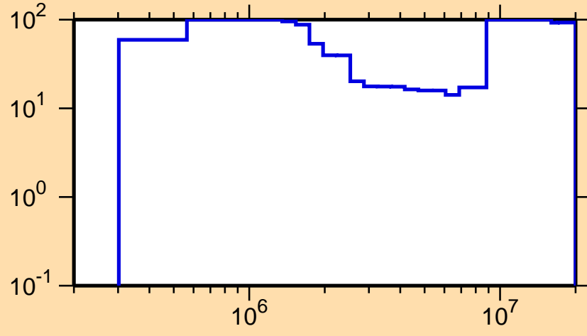
\Delta\sigma/\sigma vs. E for ^{166}\text{Lu}(n,n\text{cont.})
