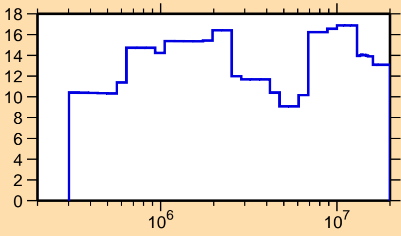
\Delta\sigma/\sigma vs. E for ^{166}\text{Lu}(n,tot.)
