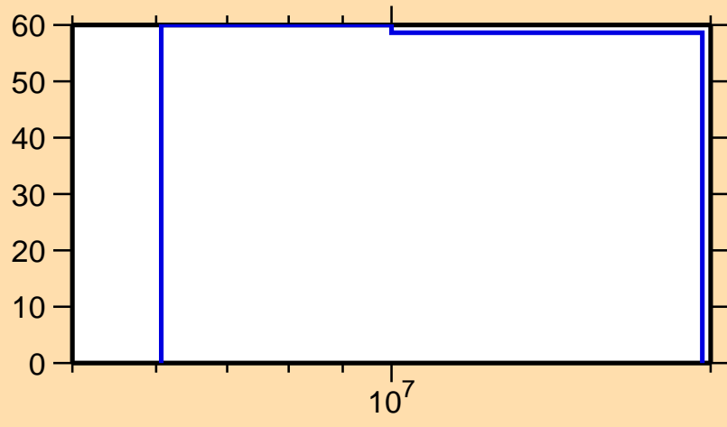
\Delta\sigma/\sigma vs. E for ^{166}\text{Lu}(n,2n)
