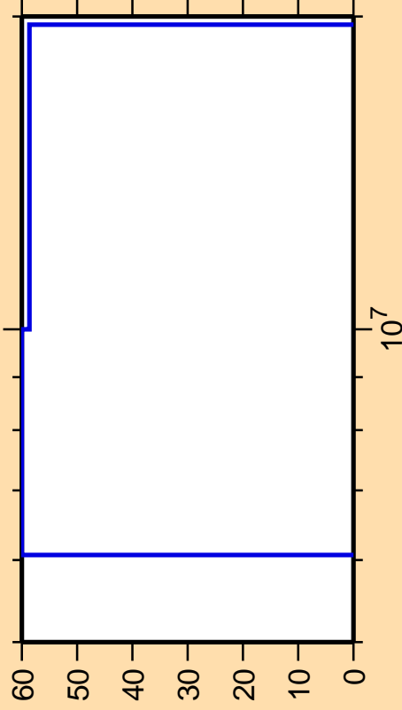
\Delta\sigma/\sigma vs. E for ^{166}\text{Lu}(n,2n)
