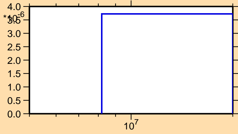
\sigma vs. E for ^{166}\text{Lu}(n,\text{nd})
