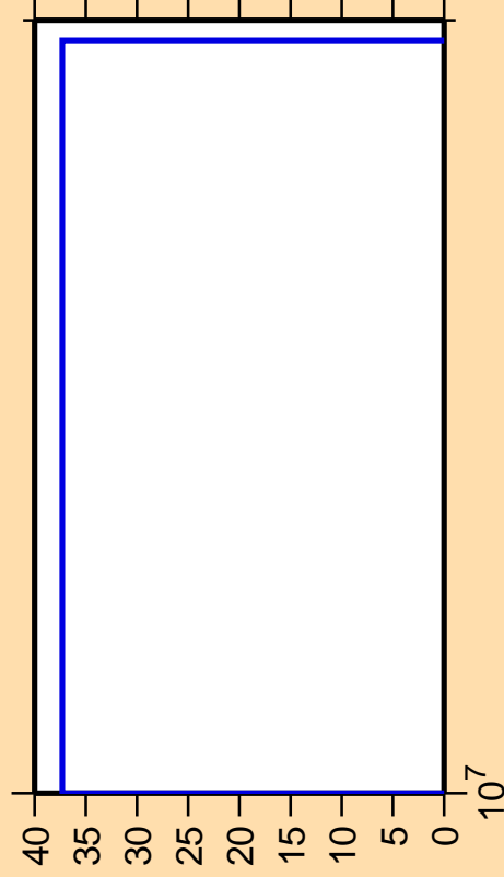
\Delta\sigma/\sigma vs. E for ^{166}\text{Lu}(n,pd)
