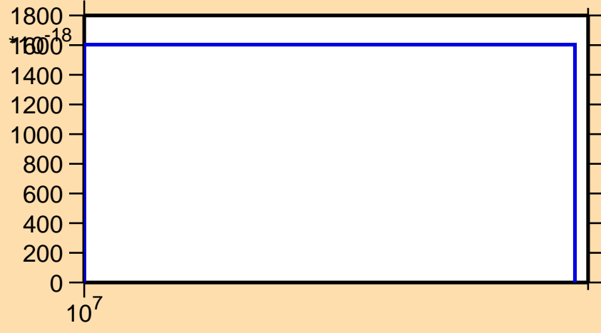
\sigma vs. E for ^{166}\text{Lu}(n,3n\alpha)
