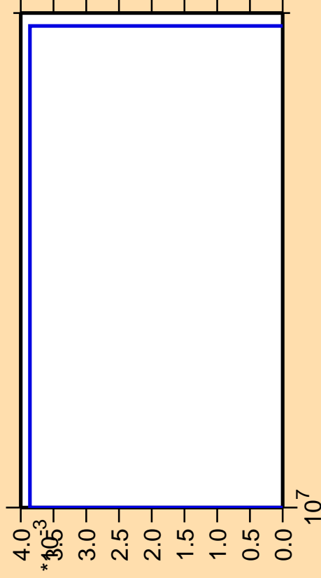
\Delta\sigma/\sigma vs. E for ^{166}\text{Lu}(n,3n\alpha)
