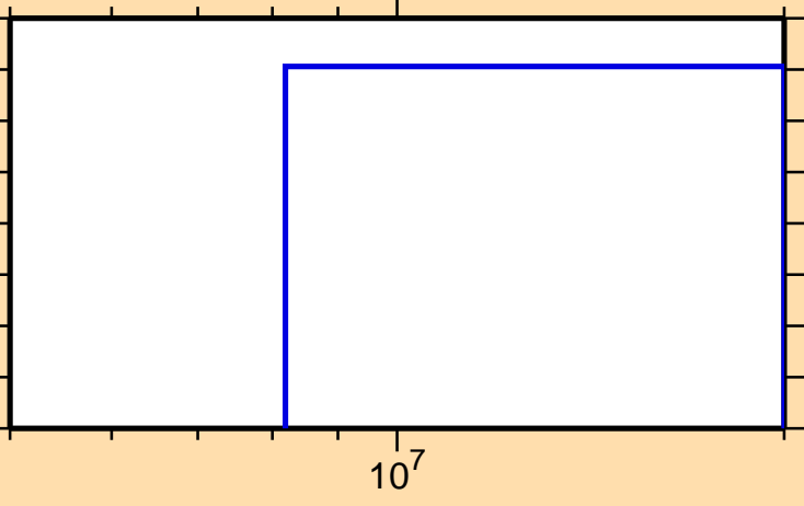
\sigma vs. E for ^{166}\text{Lu}(n,\text{nd})
