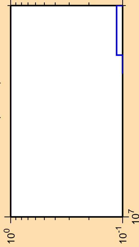
\Delta\sigma/\sigma vs. E for ^{167}\text{Lu}(n,3n\alpha)
