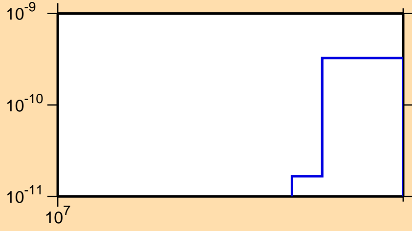
\sigma vs. E for ^{167}\text{Lu}(n,pd)
