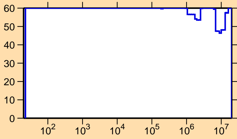
\Delta\sigma/\sigma vs. E for ^{167}\text{Lu}(n,p)
