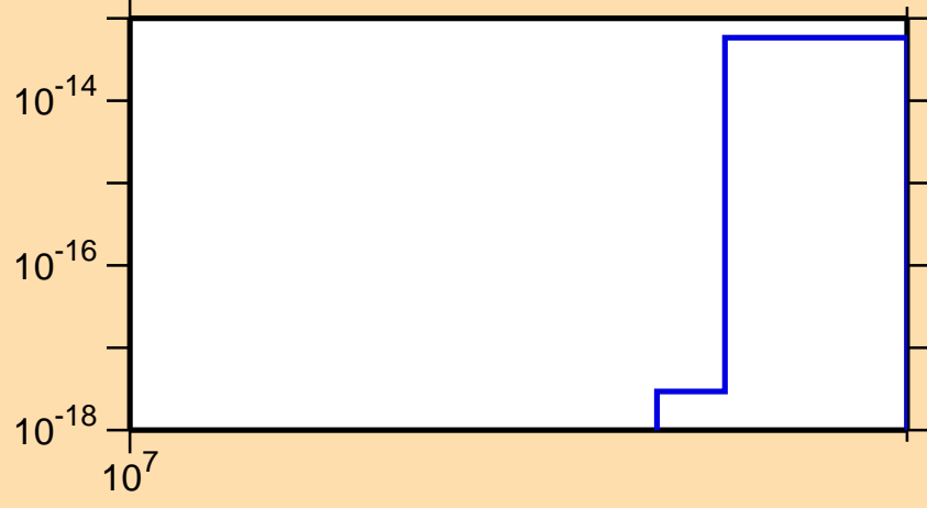
\sigma vs. E for ^{167}\text{Lu}(n,3n\alpha)
