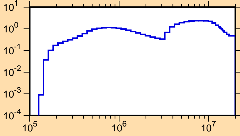
\sigma vs. E for ^{167}\text{Lu}(n,\text{inel.})
