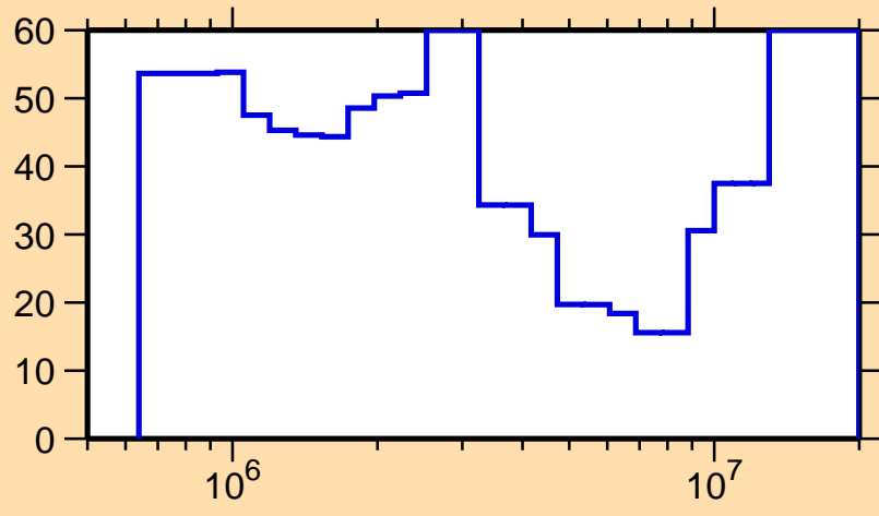
\Delta\sigma/\sigma vs. E for ^{167}\text{Lu}(n,n\text{cont.})
