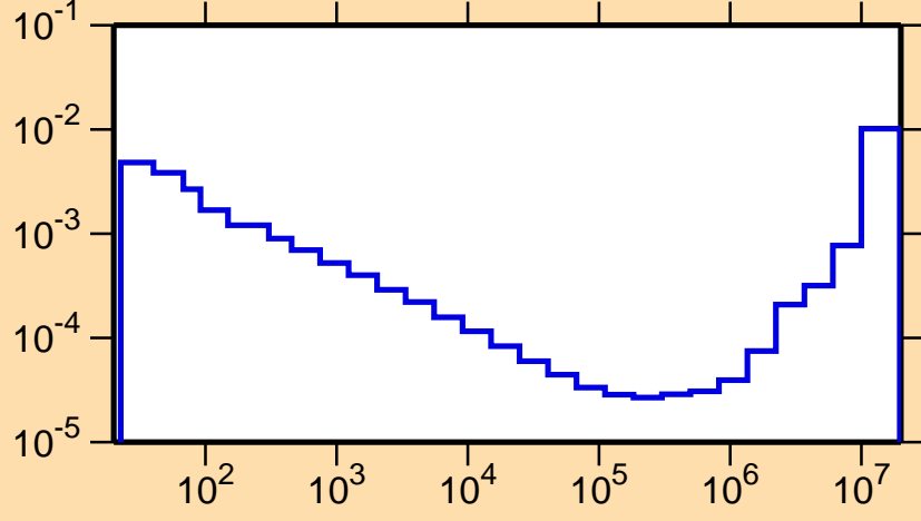
\sigma vs. E for ^{167}\text{Lu}(n,\alpha)
