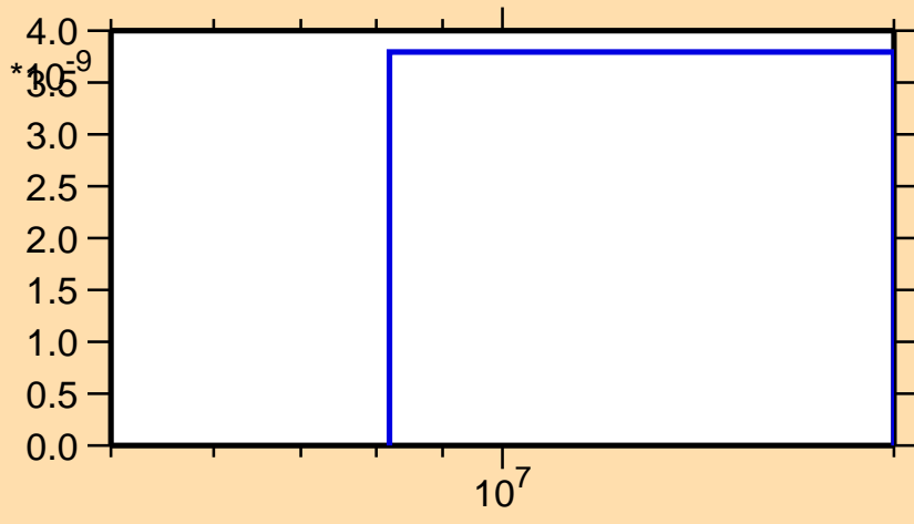
\sigma vs. E for ^{167}\text{Lu} (mt 45)
