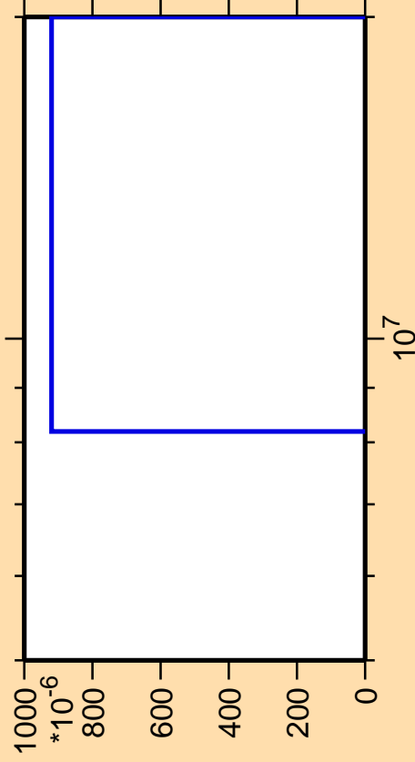
\Delta\sigma/\sigma vs. E for ^{167}\text{Lu}(n,3n\alpha)
