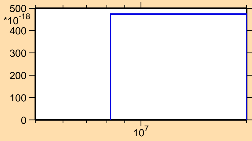
\sigma vs. E for ^{167}\text{Lu}(n,3n\alpha)
