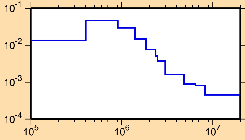
\sigma vs. E for ^{167}\text{Lu}(n,n_1)
