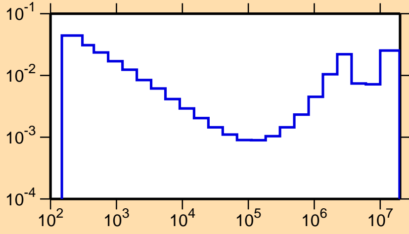
\sigma vs. E for ^{167}\text{Lu}(n,p)
