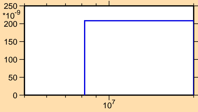
\sigma vs. E for ^{167}\text{Lu}(n,nd)
