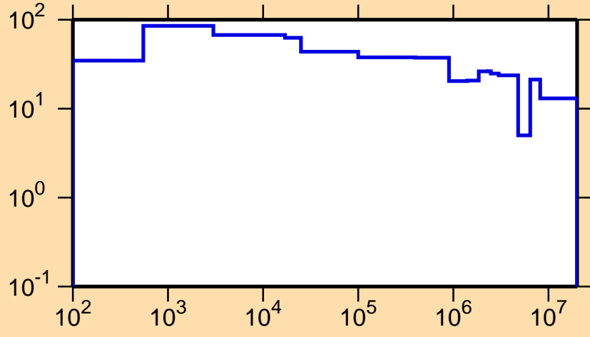
\Delta\sigma/\sigma vs. E for ^{167}\text{Lu}(n,el.)
