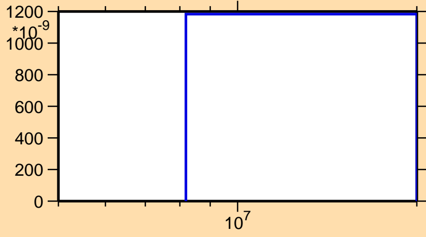
\sigma vs. E for ^{168}\text{Lu}(n,nd)
