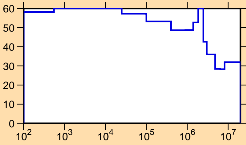
\Delta\sigma/\sigma vs. E for ^{168}\text{Lu}(n,p)
