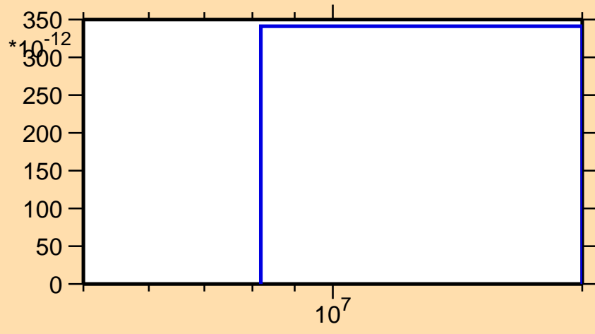
\sigma vs. E for ^{168}\text{Lu}(\text{mt } 45)
