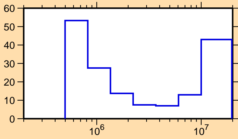
\Delta\sigma/\sigma vs. E for ^{168}\text{Lu}(n,n\text{cont.})
