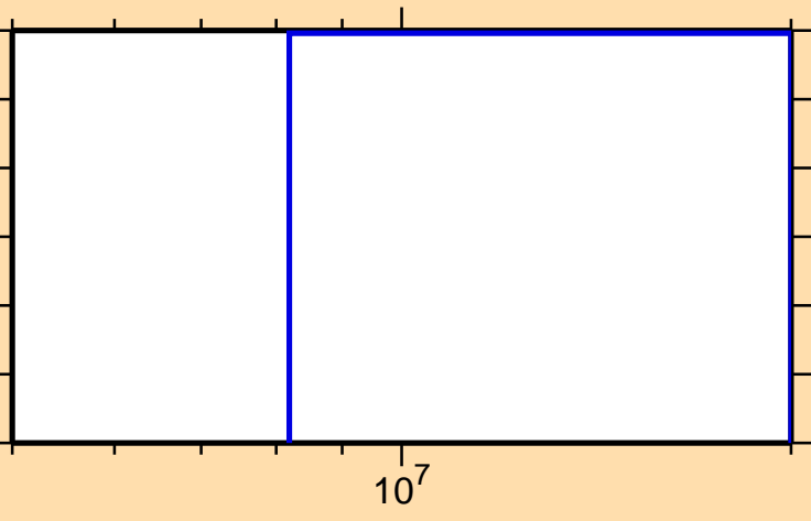
\sigma vs. E for ^{168}\text{Lu}(n,\text{He3})
