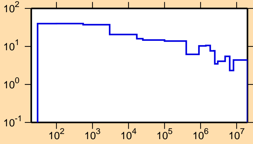
\Delta\sigma/\sigma vs. E for ^{168}\text{Lu}(n,el.)
