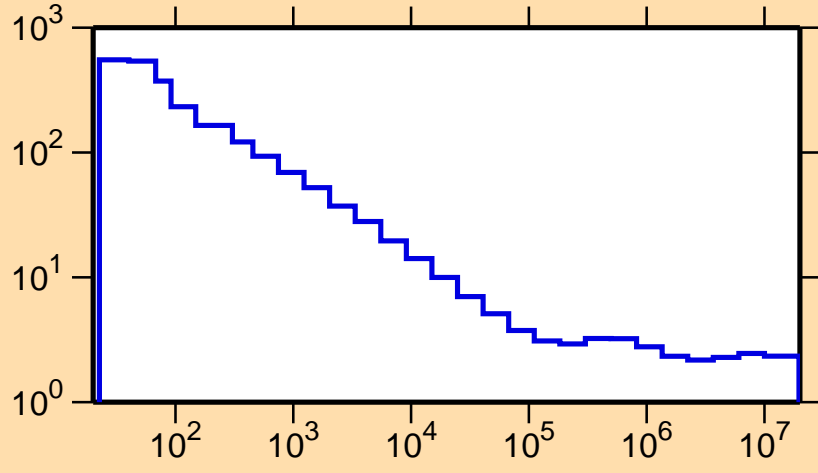
\sigma vs. E for ^{169}\text{Lu}(n,\text{nonel.})
