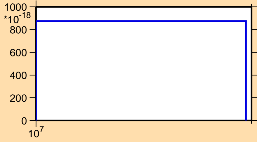
\sigma vs. E for ^{169}\text{Lu}(n,3n\alpha)
