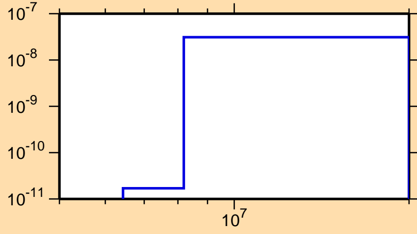
\sigma vs. E for ^{169}\text{Lu}(n,p\alpha)
