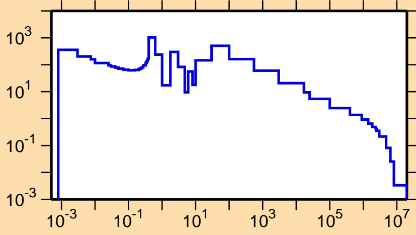
\sigma vs. E for ^{169}\text{Lu}(n,\gamma)
