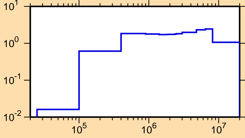
\sigma vs. E for ^{169}\text{Lu}(n,\text{inel.})
