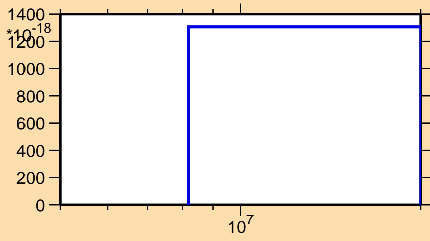
\sigma vs. E for ^{169}\text{Lu}(n,3n\alpha)
