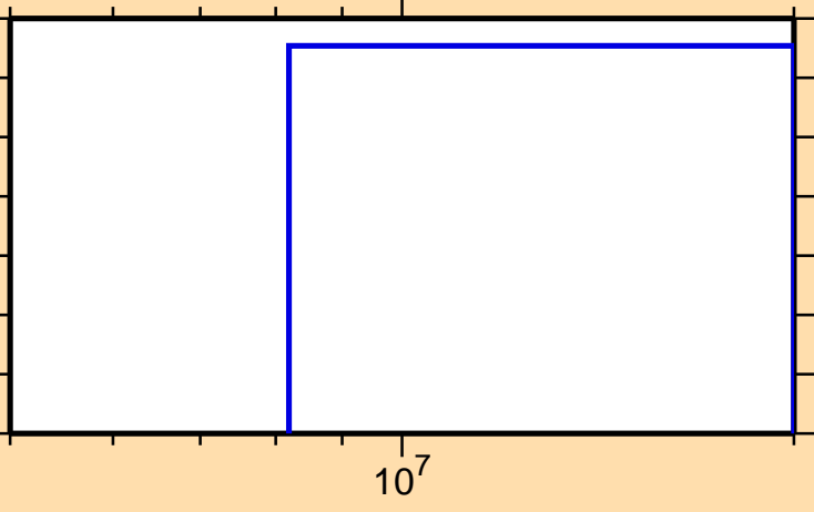
\sigma vs. E for ^{169}\text{Lu}(n,t)
