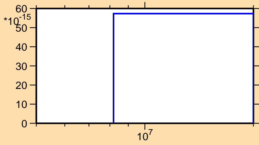
\sigma vs. E for ^{169}\text{Lu}(n,pd)
