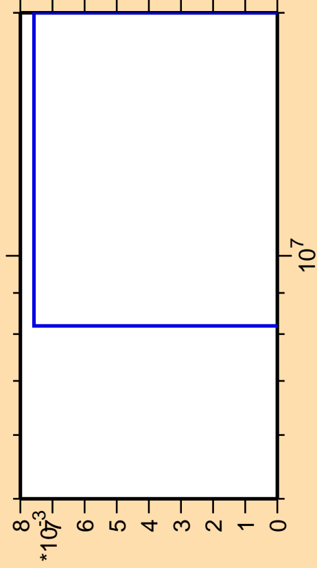
\Delta\sigma/\sigma vs. E for ^{169}\text{Lu}(n,3n\alpha)
