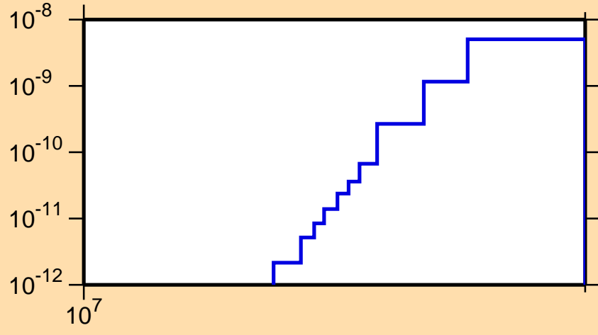
\sigma vs. E for ^{169}\text{Lu}(\text{mt117})
