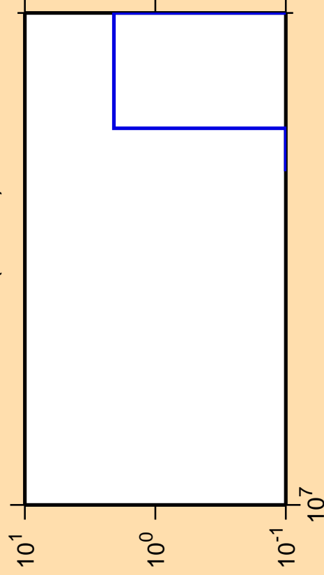
\Delta\sigma/\sigma vs. E for ^{169}\text{Lu}(n,3n\alpha)
