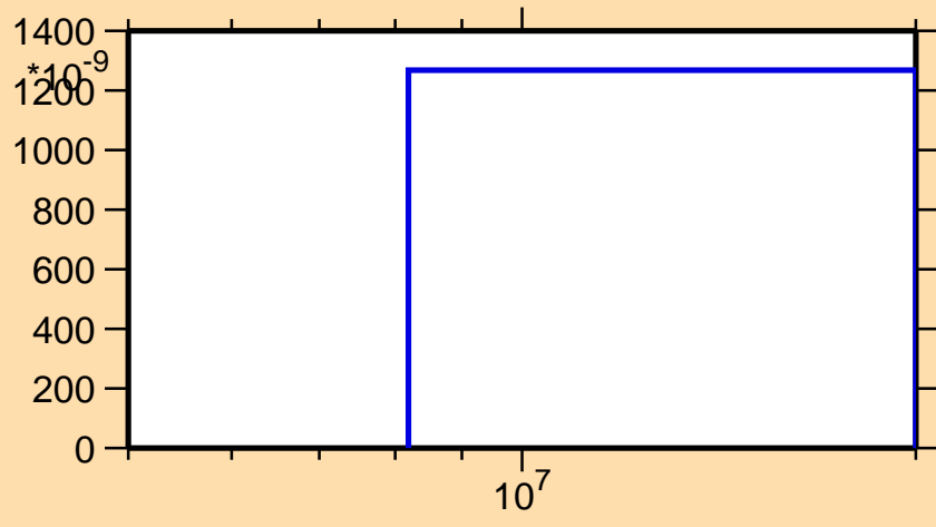
\sigma vs. E for ^{169}\text{Lu}(n,2np)
