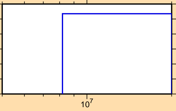
\sigma vs. E for ^{169}\text{Lu}(n,nt)
