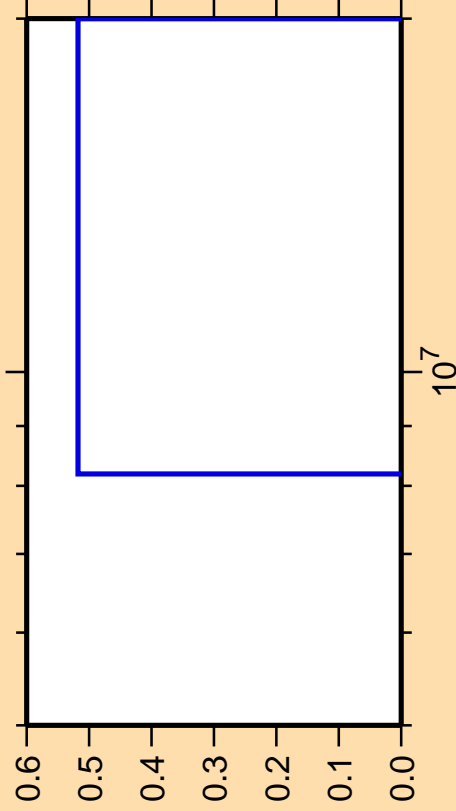
\Delta\sigma/\sigma vs. E for ^{169}\text{Lu}(n,pd)
