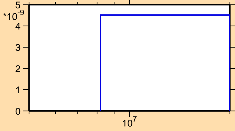
\sigma vs. E for ^{169}\text{Lu}(n,\text{He3})
