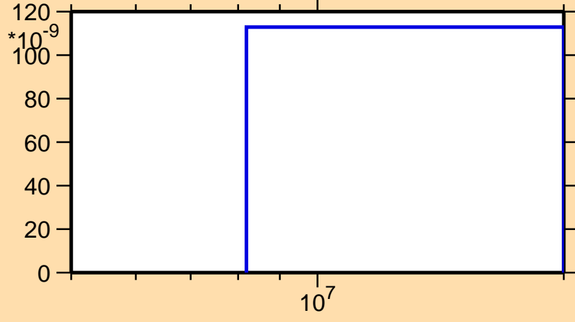
\sigma vs. E for ^{169}\text{Lu}(n,nd)
