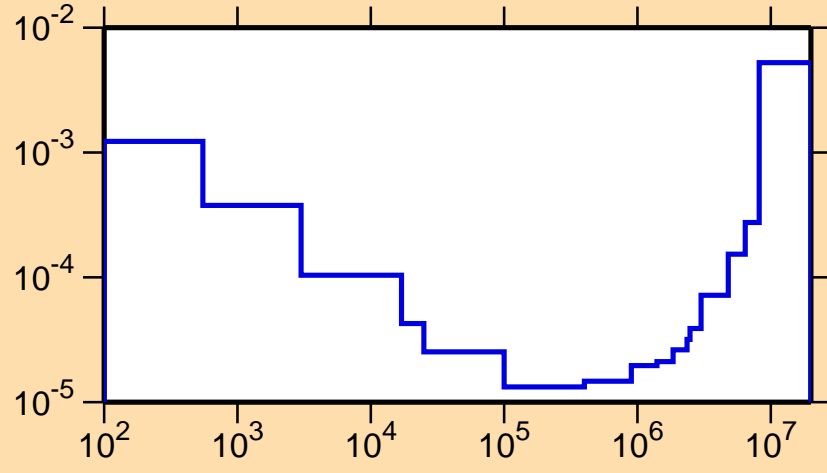
\sigma vs. E for ^{169}\text{Lu}(n,\alpha)
