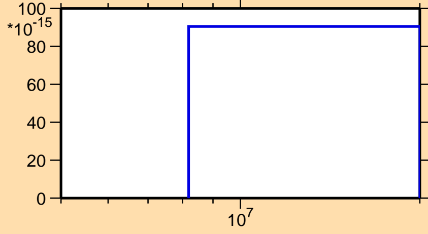
\sigma vs. E for ^{169}\text{Lu}(n,pd)
