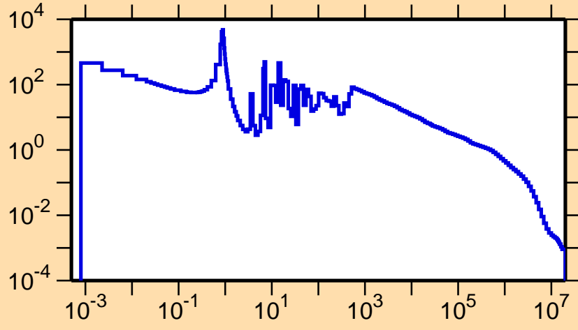
\sigma vs. E for ^{170}\text{Lu}(n,\gamma)
