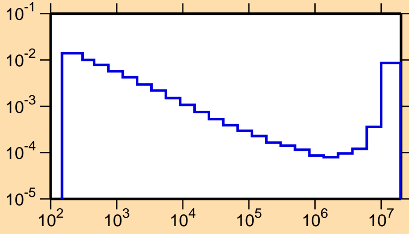
\sigma vs. E for ^{170}\text{Lu}(n,\alpha)
