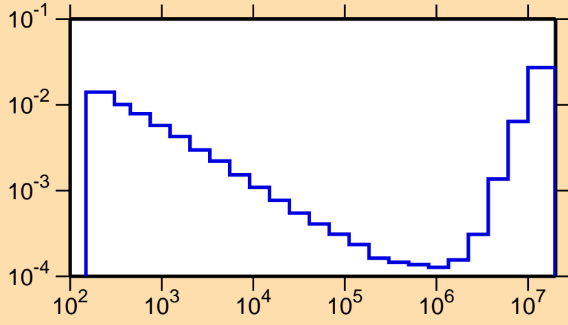
\sigma vs. E for ^{170}\text{Lu}(n,p)
