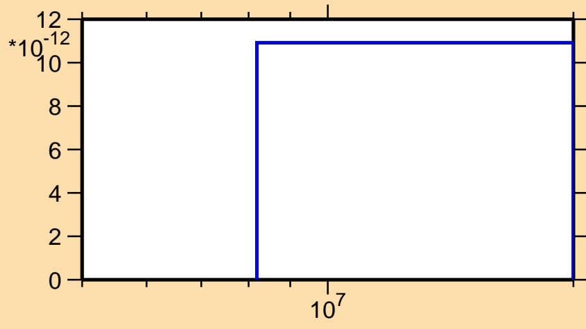
\sigma vs. E for ^{170}\text{Lu}(\text{mt117})
