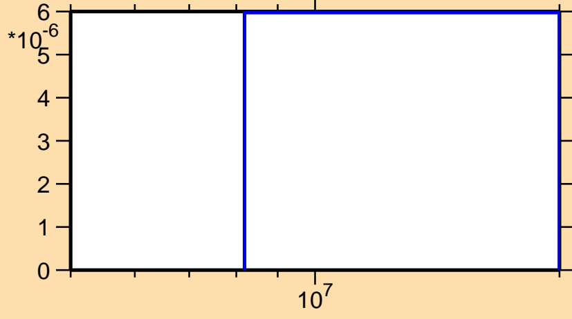
\sigma vs. E for ^{170}\text{Lu}(n,2n\alpha)
