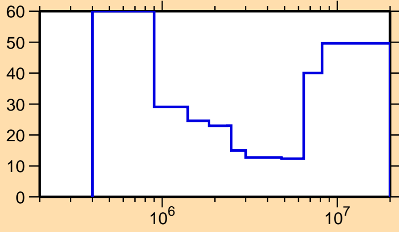
\Delta\sigma/\sigma vs. E for ^{170}\text{Lu}(n,n\text{cont.})
