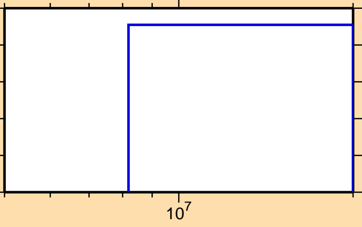
\sigma vs. E for ^{170}\text{Lu}(n,\text{pt})
