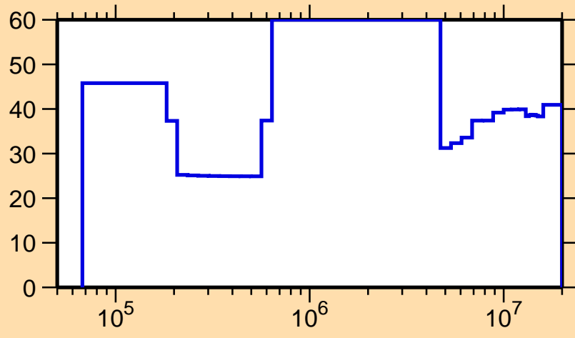
\Delta\sigma/\sigma vs. E for ^{171}\text{Lu}(n,n_1)
