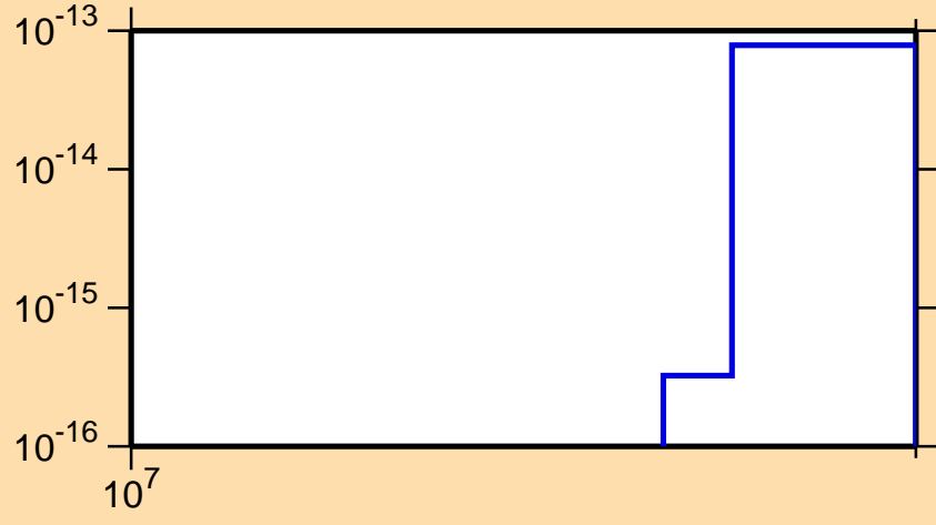
\sigma vs. E for ^{171}\text{Lu}(n,pd)
