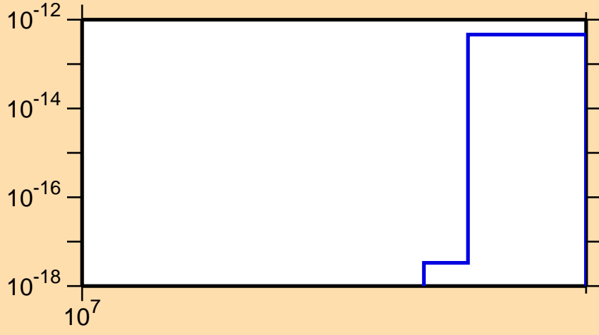
\sigma vs. E for ^{171}\text{Lu}(n,3n\alpha)
