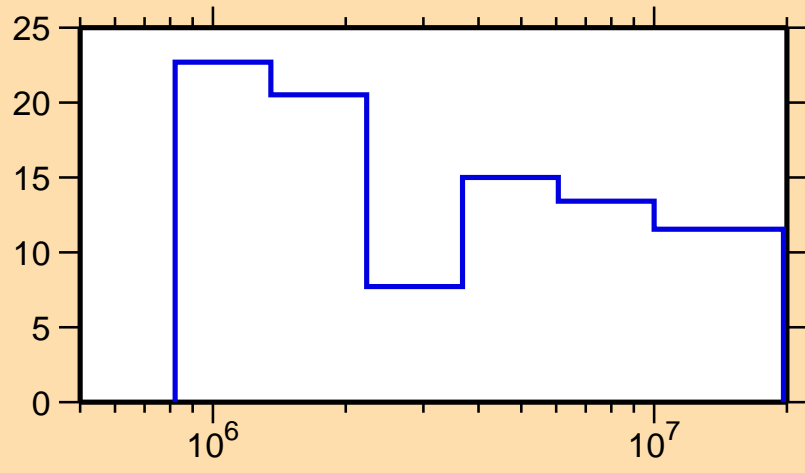
\Delta\sigma/\sigma vs. E for ^{171}\text{Lu}(n,el.)
