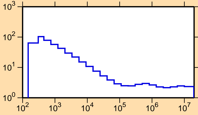
\sigma vs. E for ^{171}\text{Lu}(n,\text{nonel.})
