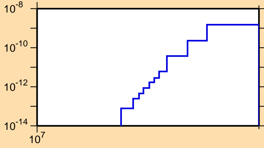
\sigma vs. E for ^{171}\text{Lu} (mt 45)
