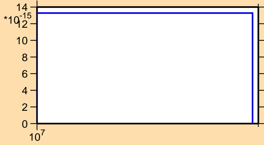
\sigma vs. E for ^{171}\text{Lu}(n,3n\alpha)
