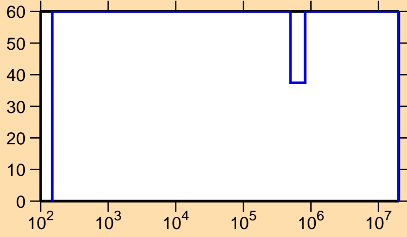
\Delta\sigma/\sigma vs. E for ^{171}\text{Lu}(n,p)
