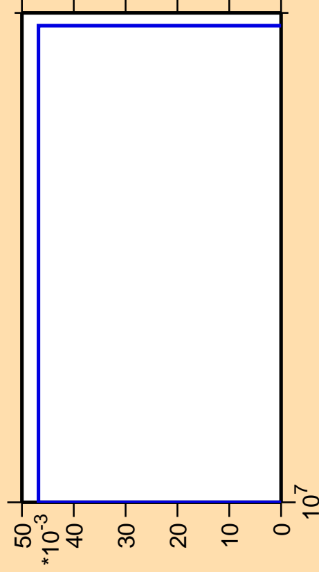
\Delta\sigma/\sigma vs. E for ^{171}\text{Lu}(n,3n\alpha)
