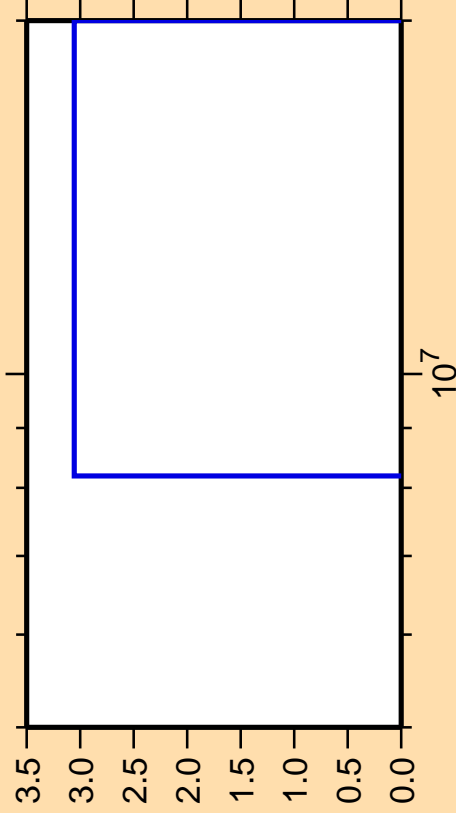
\Delta\sigma/\sigma vs. E for ^{172}\text{Lu}(\text{mt } 45)
