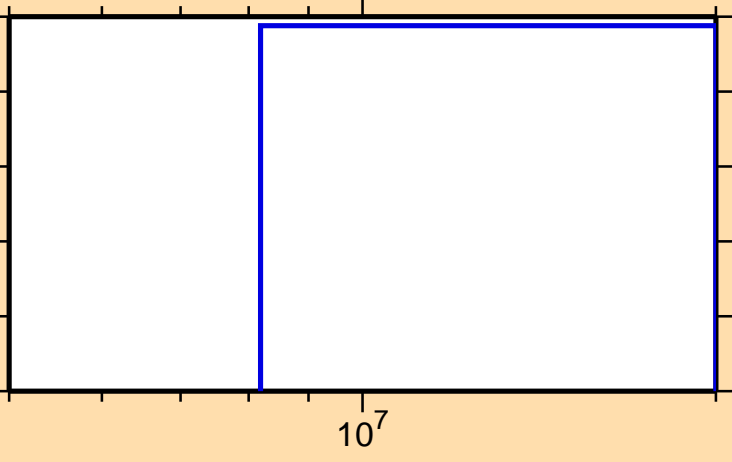
\sigma vs. E for ^{172}\text{Lu}(n,\text{nd})
