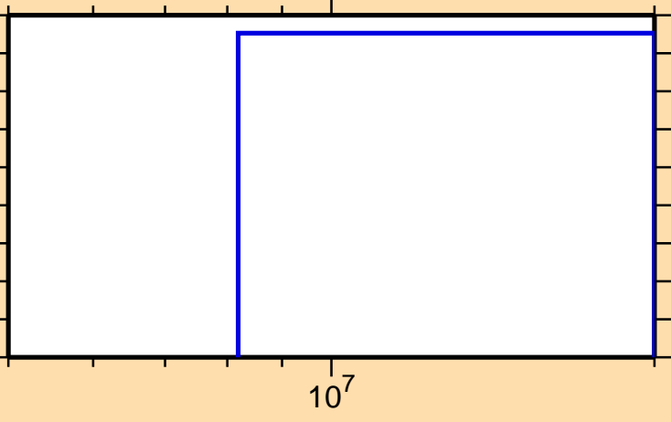
\sigma vs. E for ^{172}\text{Lu}(n,\text{He3})
