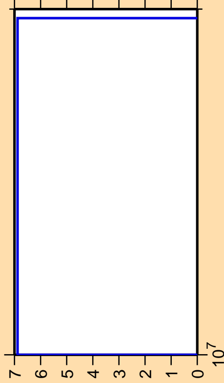
\Delta\sigma/\sigma vs. E for ^{172}\text{Lu}(n,3n)
