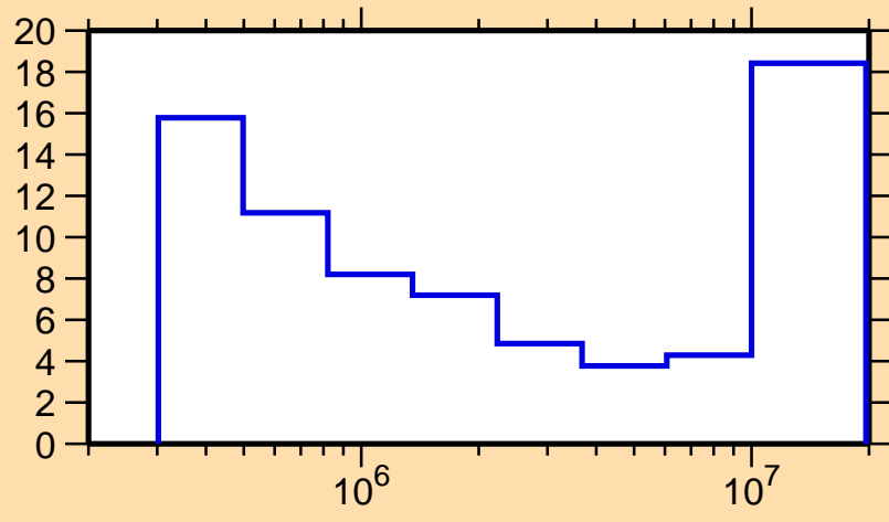
\Delta\sigma/\sigma vs. E for ^{172}\text{Lu}(n,n\text{cont.})
