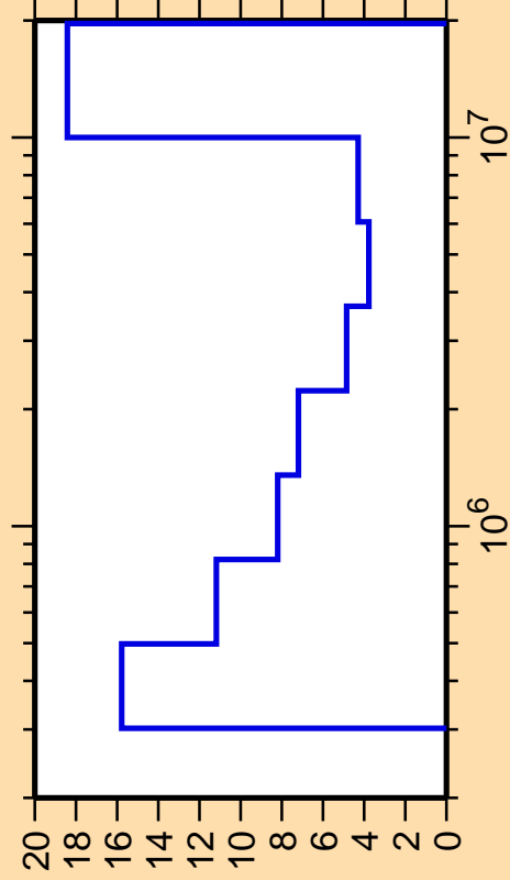
\Delta\sigma/\sigma vs. E for ^{172}\text{Lu}(n,\text{ncont.})
