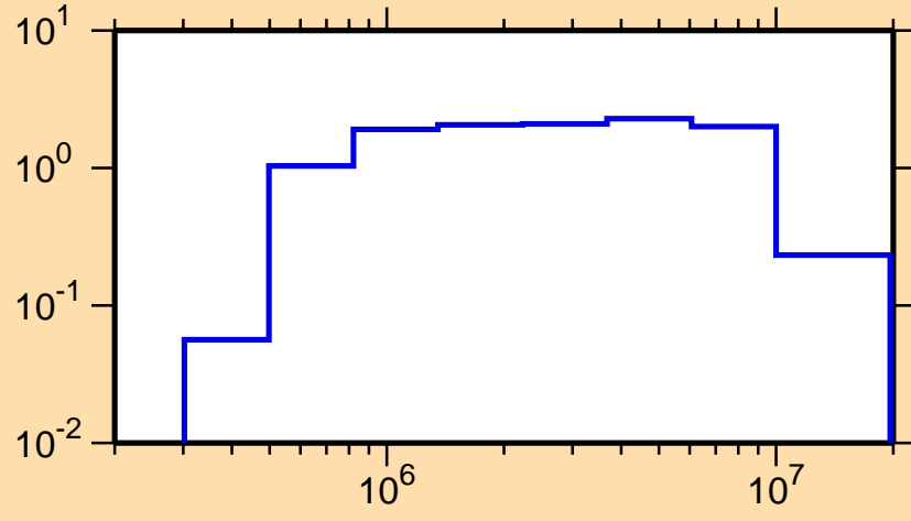
\sigma vs. E for ^{172}\text{Lu}(n,n\text{cont.})
