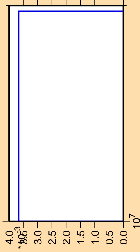
\Delta\sigma/\sigma vs. E for ^{172}\text{Lu}(n,3n\alpha)
