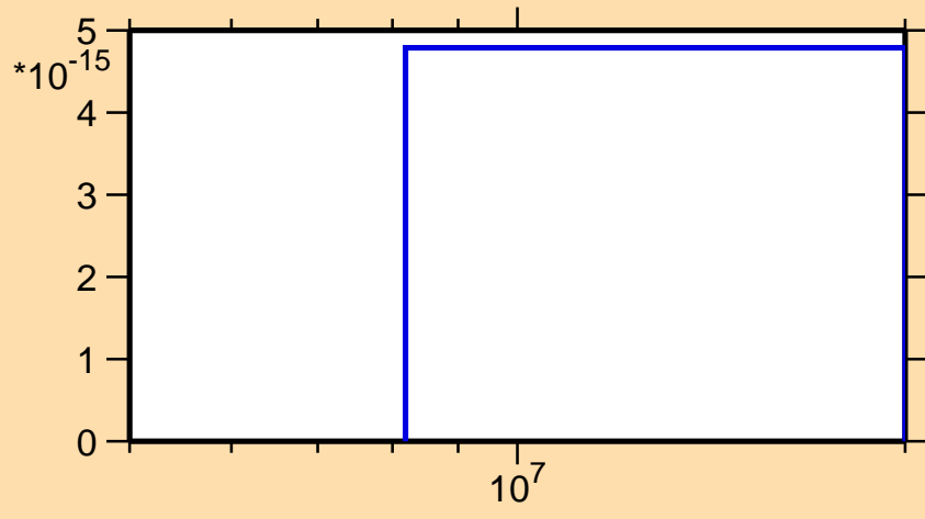
\sigma vs. E for ^{172}\text{Lu}(n,3n\alpha)
