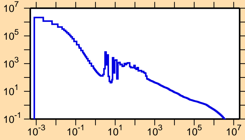
\sigma vs. E for ^{173}\text{Lu}(n,\gamma)
