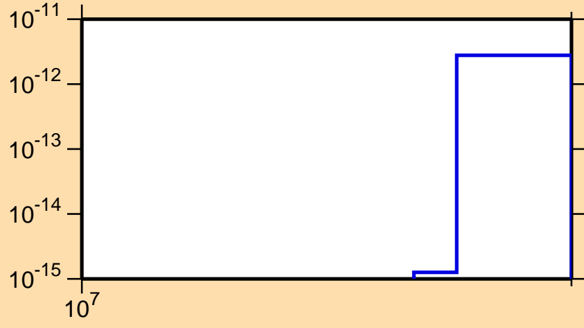
\sigma vs. E for ^{173}\text{Lu}(n,3n\alpha)
