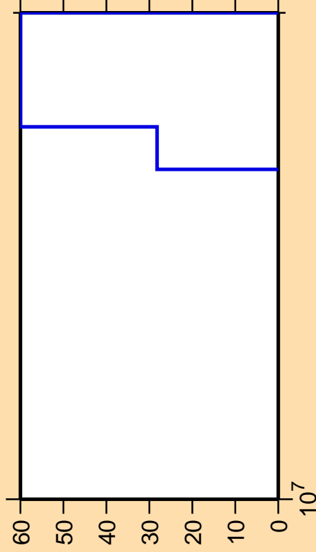
\Delta\sigma/\sigma vs. E for ^{173}\text{Lu}(\text{mt117})
