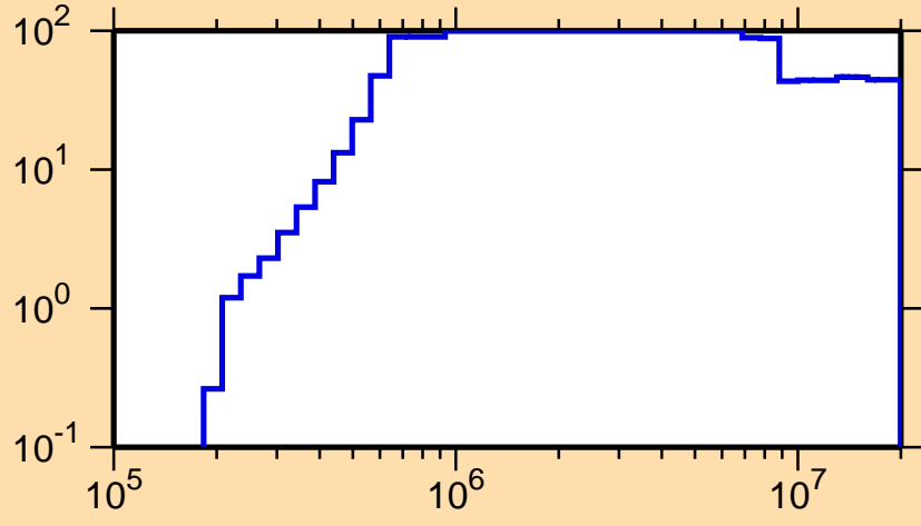
\Delta\sigma/\sigma vs. E for ^{173}\text{Lu}(n,p)
