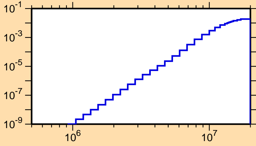
\sigma vs. E for ^{173}\text{Lu}(n,p)
