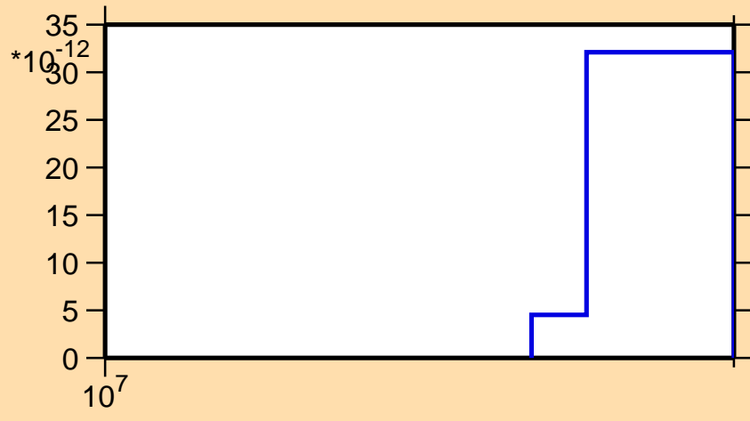
\sigma vs. E for ^{173}\text{Lu}(\text{mt117})
