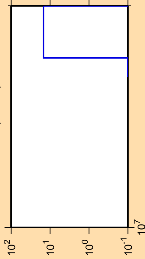
\Delta\sigma/\sigma vs. E for ^{173}\text{Lu}(n,3n\alpha)
