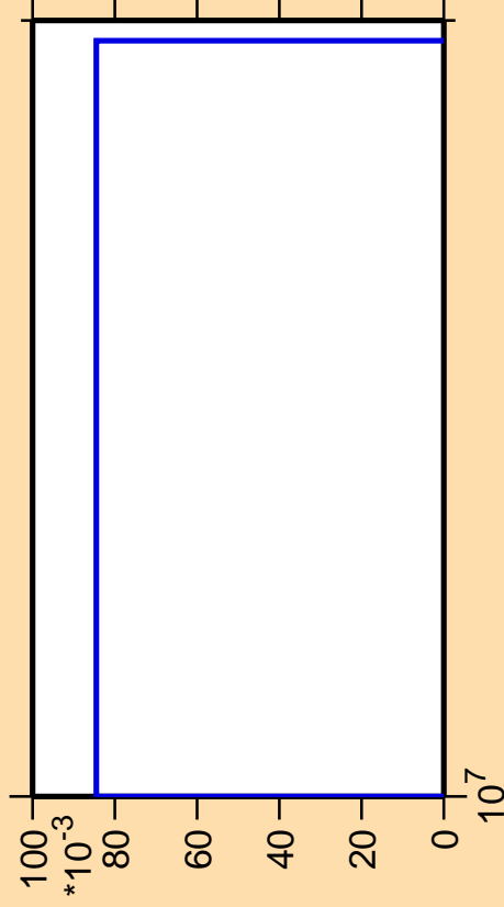
\Delta\sigma/\sigma vs. E for ^{173}\text{Lu}(n,3n\alpha)
