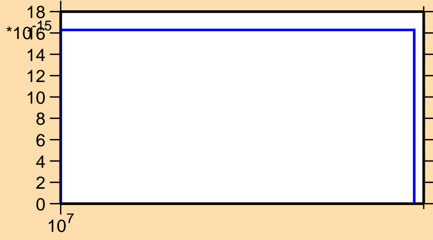
\sigma vs. E for ^{173}\text{Lu}(n,3n\alpha)
