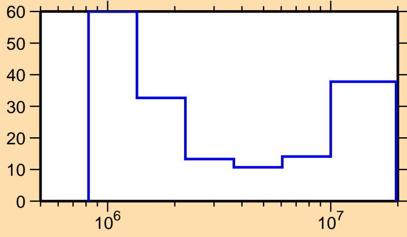
\Delta\sigma/\sigma vs. E for ^{173}\text{Lu}(n,n\text{cont.})
