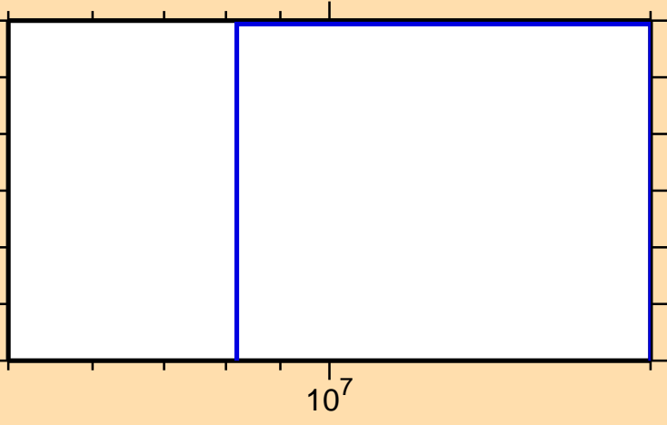
\sigma vs. E for ^{173}\text{Lu}(n,3n)
