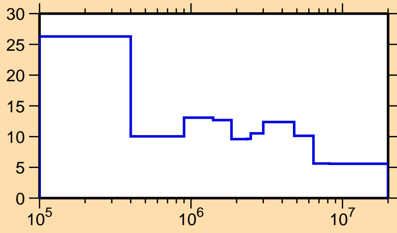
\Delta\sigma/\sigma vs. E for ^{173}\text{Lu}(n,el.)
