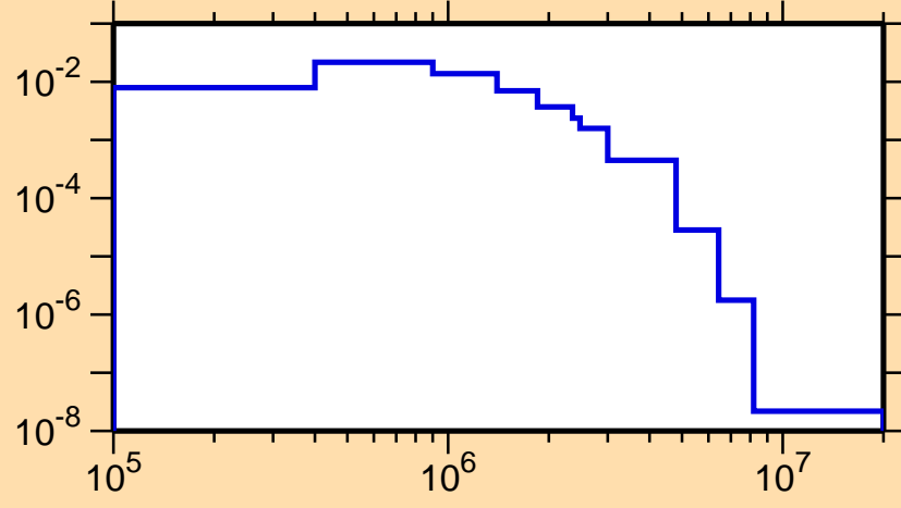
\sigma vs. E for ^{173}\text{Lu}(n,n_3)
