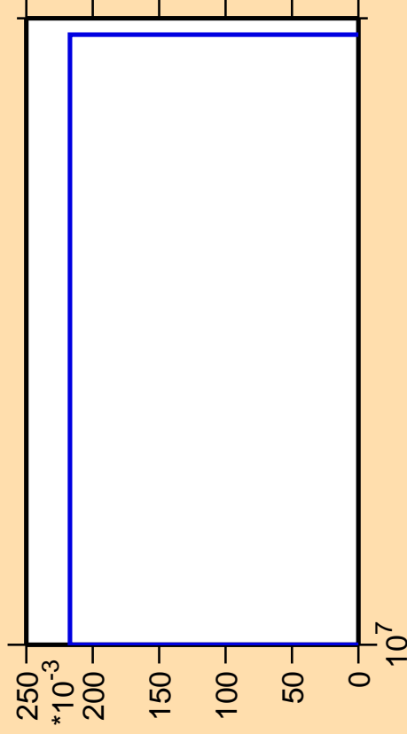
\Delta\sigma/\sigma vs. E for ^{174}\text{Lu}(\text{mt117})
