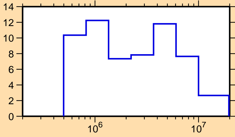
\Delta\sigma/\sigma vs. E for ^{174}\text{Lu}(n,\text{tot.})
