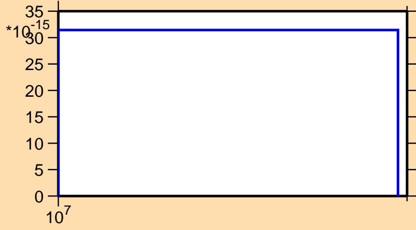
\sigma vs. E for ^{174}\text{Lu}(\text{mt117})
