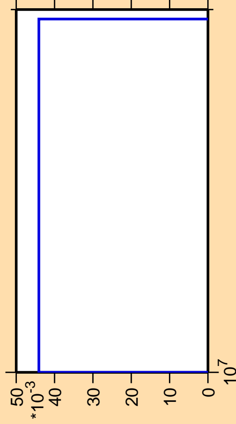
\Delta\sigma/\sigma vs. E for ^{174}\text{Lu}(n,3n\alpha)
