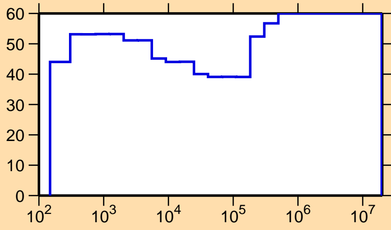
\Delta\sigma/\sigma vs. E for ^{174}\text{Lu}(n,\gamma)
