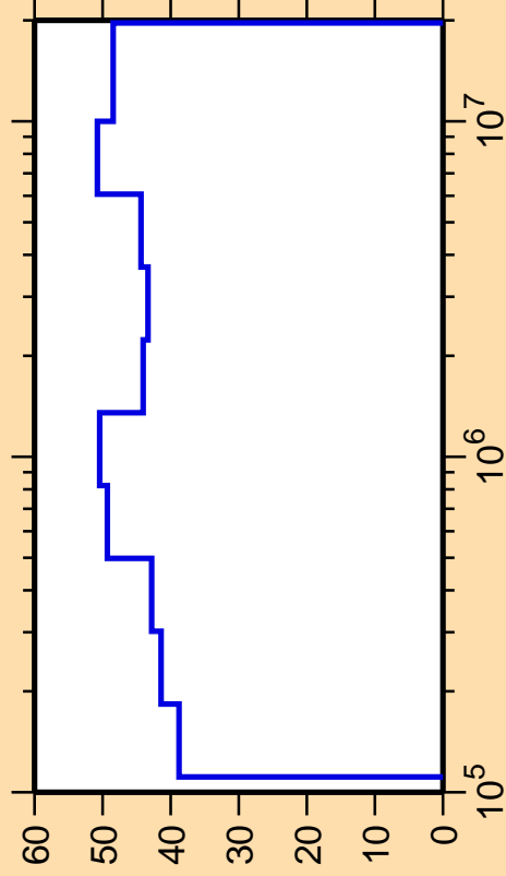
\Delta\sigma/\sigma vs. E for ^{174}\text{Lu}(n,n_2)
