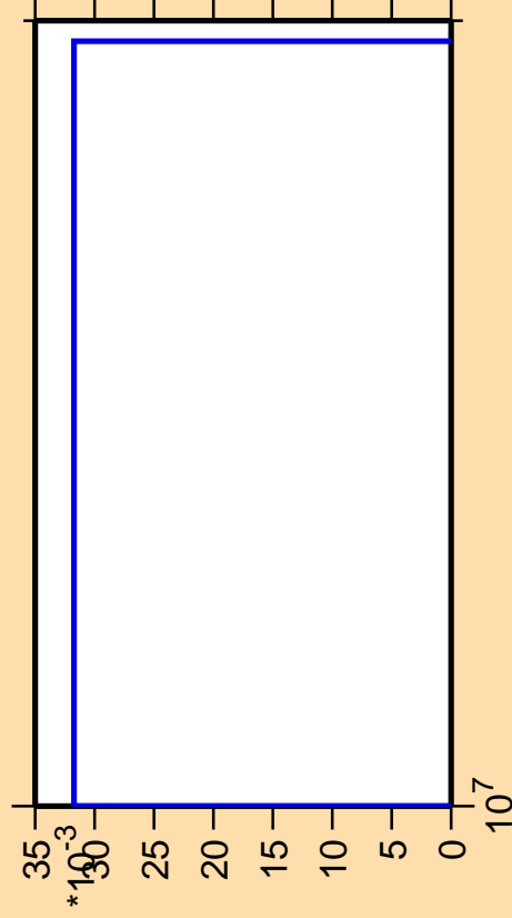
\Delta\sigma/\sigma vs. E for ^{174}\text{Lu} (mt 45)
