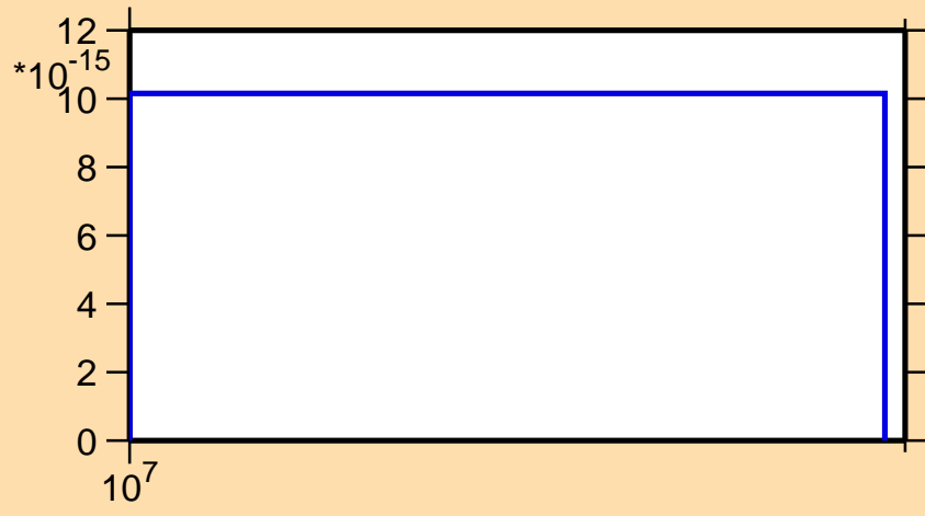
\sigma vs. E for ^{174}\text{Lu}(n,3n\alpha)
