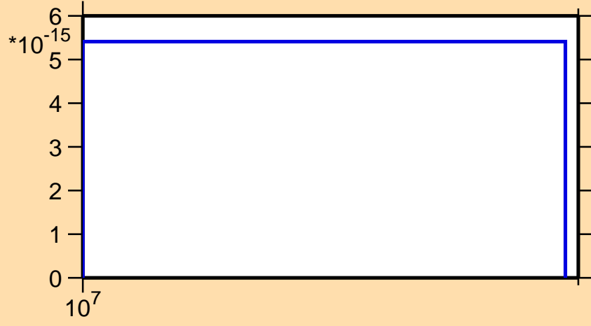
\sigma vs. E for ^{174}\text{Lu} (mt 45)
