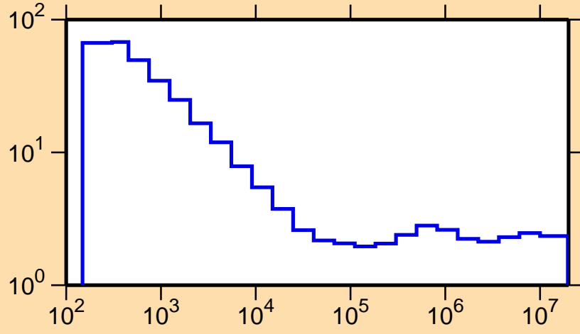
\sigma vs. E for ^{174}\text{Lu}(n,\text{nonel.})
