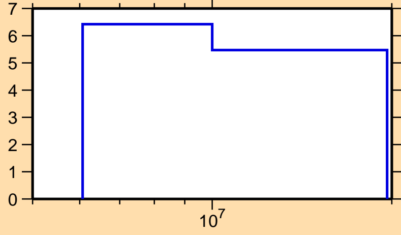
\Delta\sigma/\sigma vs. E for ^{174}\text{Lu}(n,\text{nonel.})
