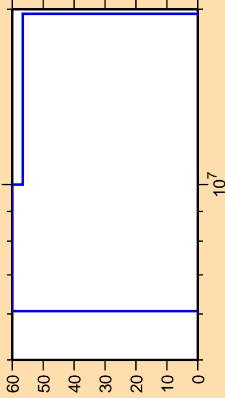
\Delta\sigma/\sigma vs. E for ^{174}\text{Lu}(n,np)
