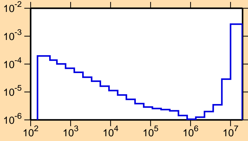
\sigma vs. E for ^{174}\text{Lu}(n,\alpha)
