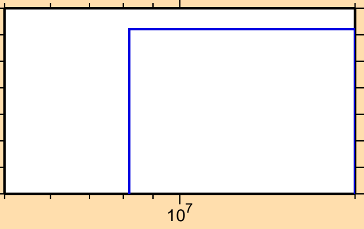
\sigma vs. E for ^{174}\text{Lu}(n,nt)
