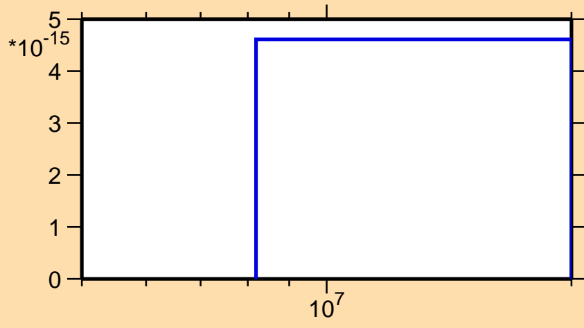
\sigma vs. E for ^{174}\text{Lu} (mt 45)
