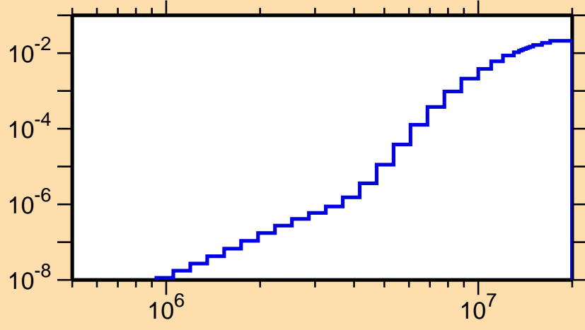
\sigma vs. E for ^{174}\text{Lu}(n,p)
