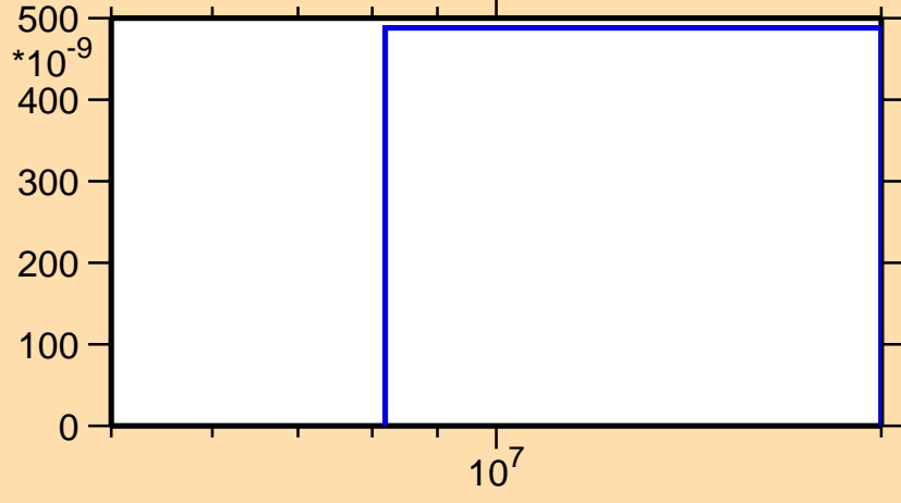
\sigma vs. E for ^{174}\text{Lu}(n,nd)
