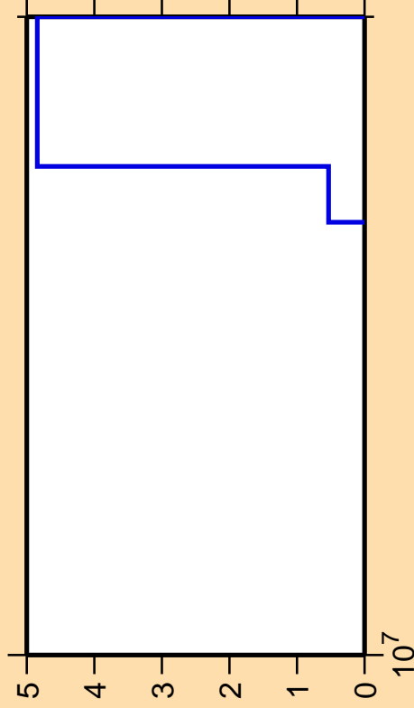
\Delta\sigma/\sigma vs. E for ^{175}\text{Lu}(\text{mt117})
