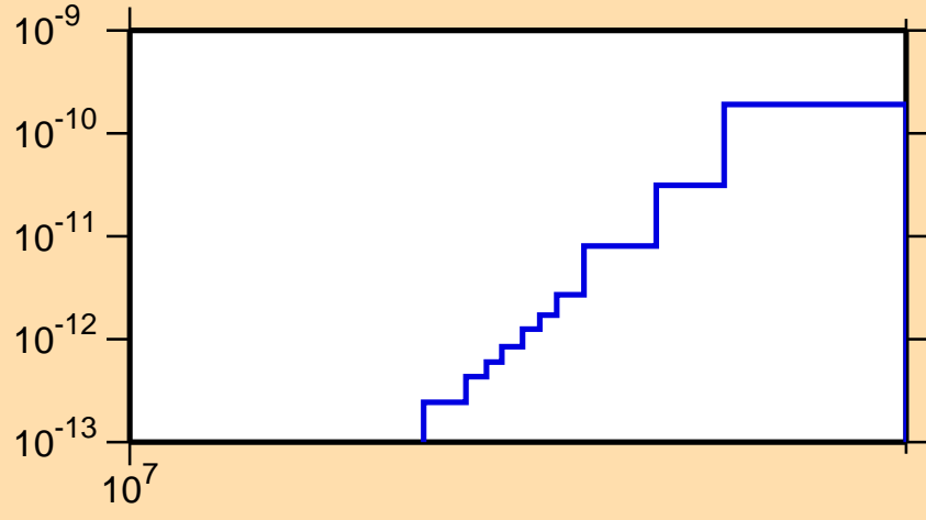
\sigma vs. E for ^{175}\text{Lu}(n,p\alpha)
