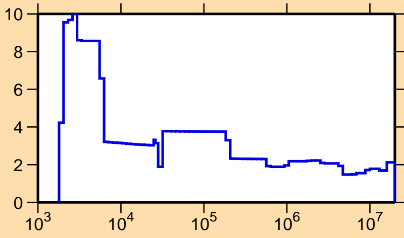
\Delta\sigma/\sigma vs. E for ^{175}\text{Lu}(n,\text{tot.})
