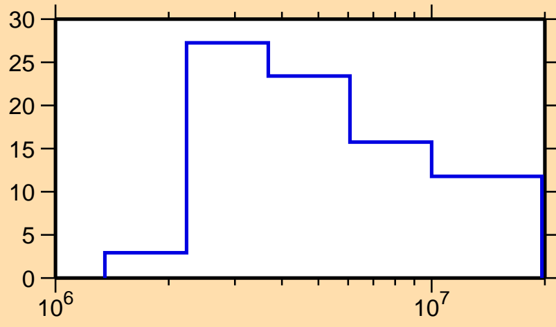
\Delta\sigma/\sigma vs. E for ^{175}\text{Lu}(n,p)
