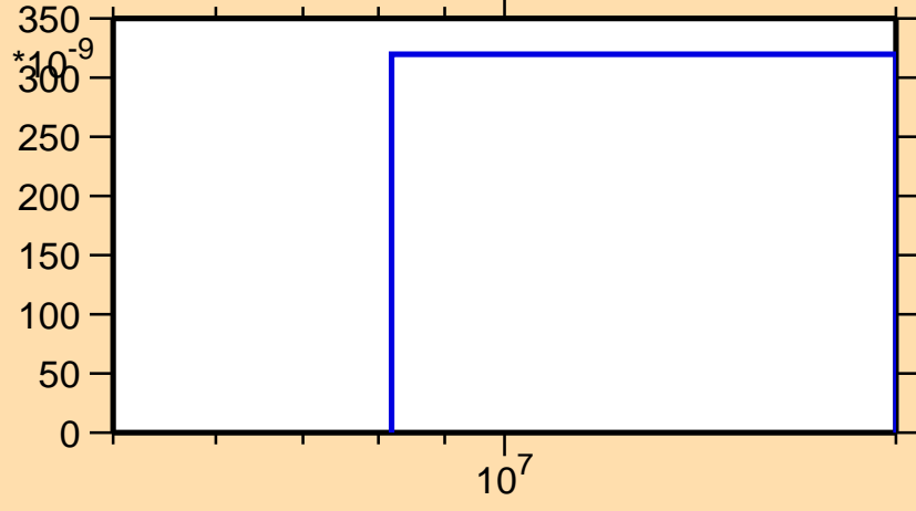
\sigma vs. E for ^{176}\text{Lu}(n,nd)
