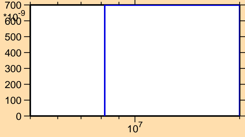
\sigma vs. E for ^{176}\text{Lu}(n,2n\alpha)
