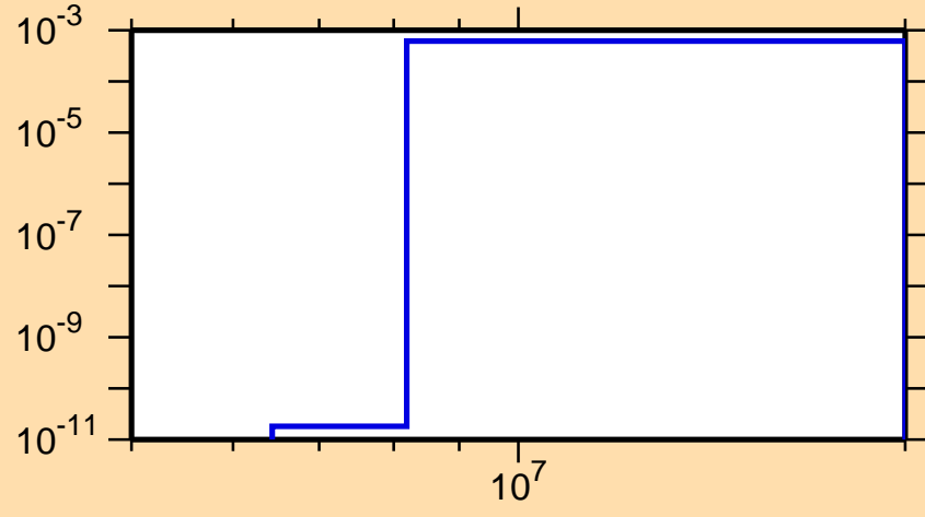
\sigma vs. E for ^{176}\text{Lu}(n,d)
