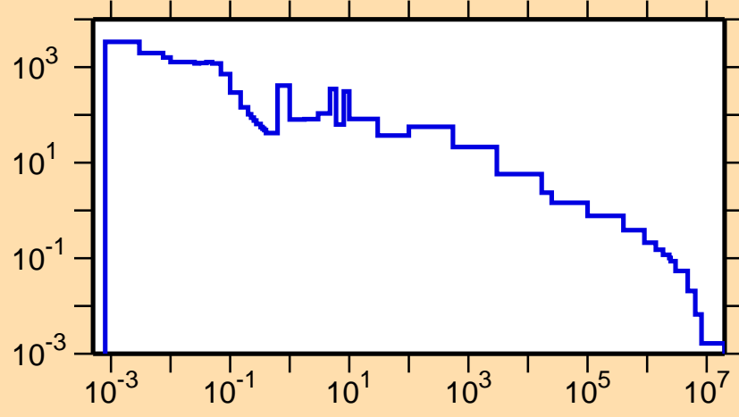
\sigma vs. E for ^{177}\text{Lu}(n,\gamma)
