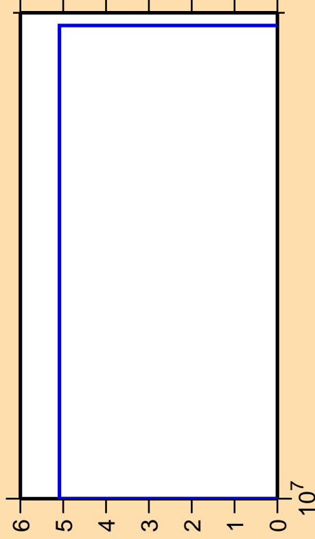
\Delta\sigma/\sigma vs. E for ^{177}\text{Lu}(n,3n\alpha)
