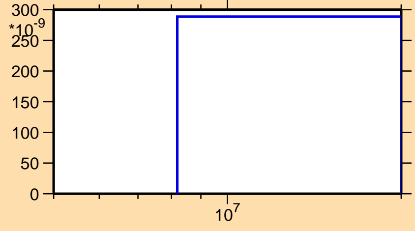
\sigma vs. E for ^{177}\text{Lu}(n,2n\alpha)
