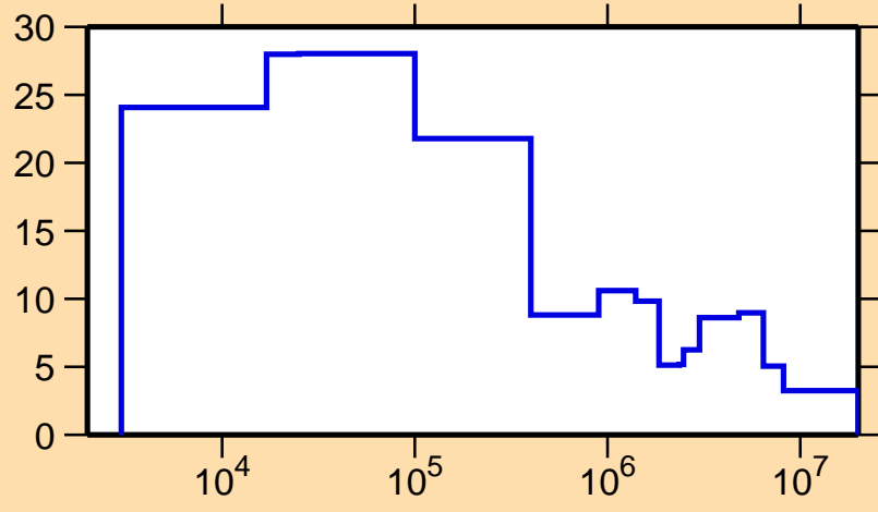
\Delta\sigma/\sigma vs. E for ^{177}\text{Lu}(n, tot.)
