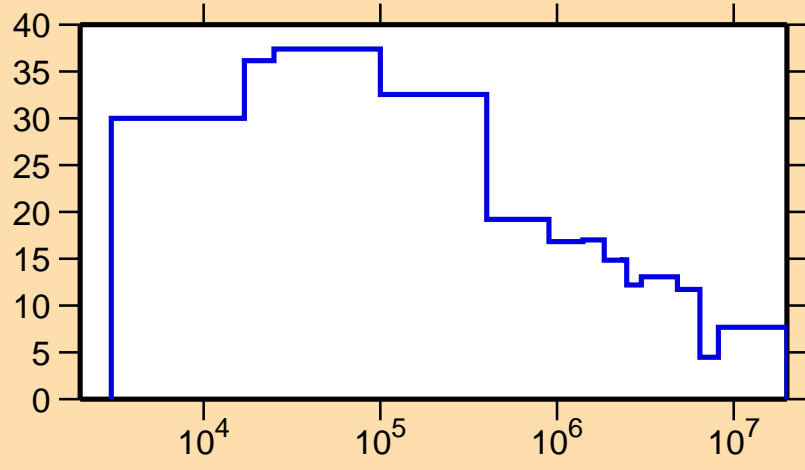
\Delta\sigma/\sigma vs. E for ^{177}\text{Lu}(n, el.)
