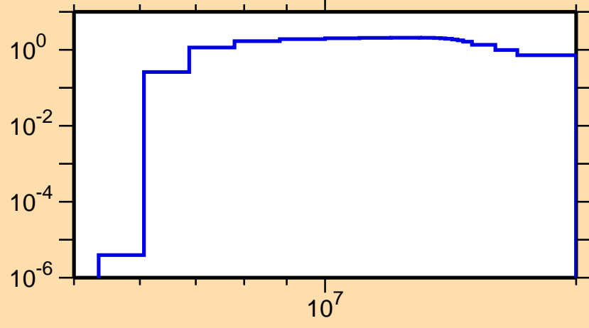
\sigma vs. E for ^{178}\text{Lu}(n,2n)
