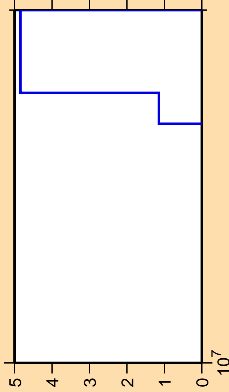
\Delta\sigma/\sigma vs. E for ^{178}\text{Lu}(n,p\alpha)
