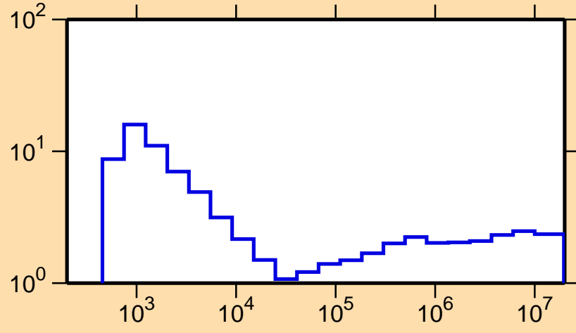
\sigma vs. E for ^{178}\text{Lu}(n,\text{nonel.})
