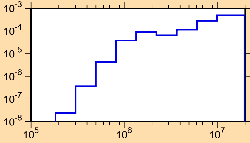
\sigma vs. E for ^{178}\text{Lu}(n,n_3)
