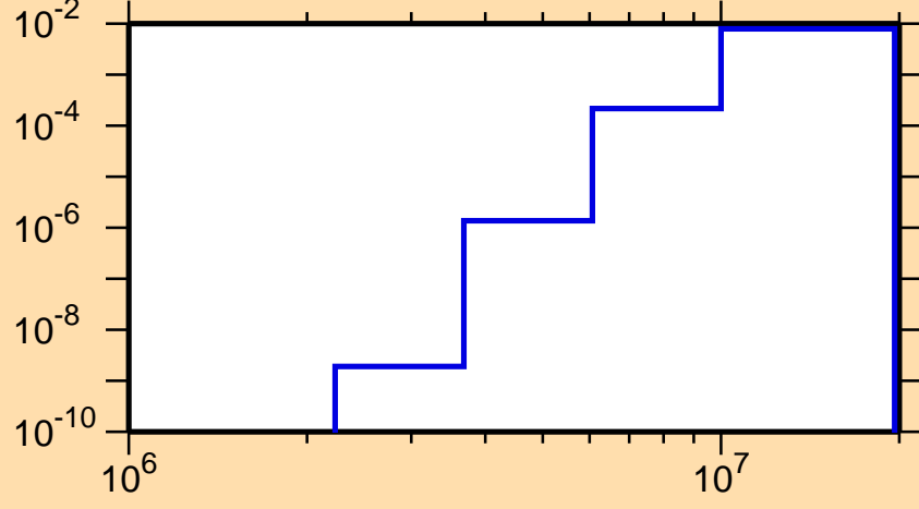
\sigma vs. E for ^{178}\text{Lu}(n,p)
