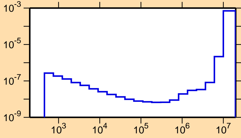
\sigma vs. E for ^{178}\text{Lu}(n,\alpha)
