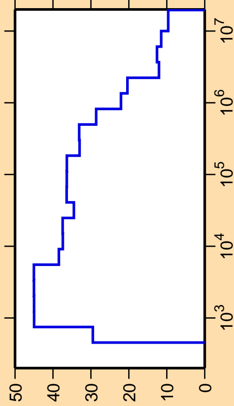
\Delta\sigma/\sigma vs. E for ^{178}\text{Lu}(n,\text{nonel.})
