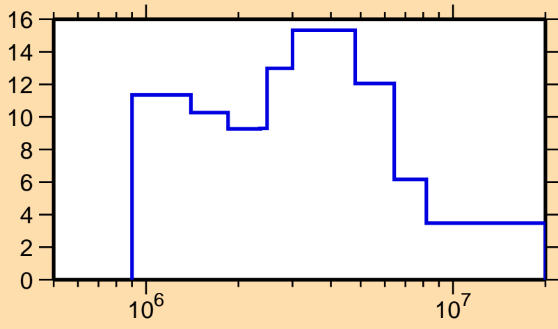
\Delta\sigma/\sigma vs. E for ^{178}\text{Lu}(n,tot.)
