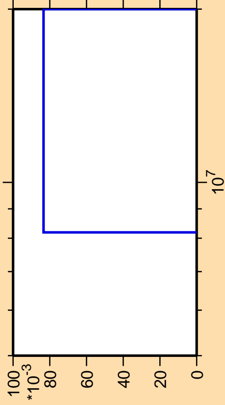
\Delta\sigma/\sigma vs. E for ^{178}\text{Lu}(n,p\alpha)
