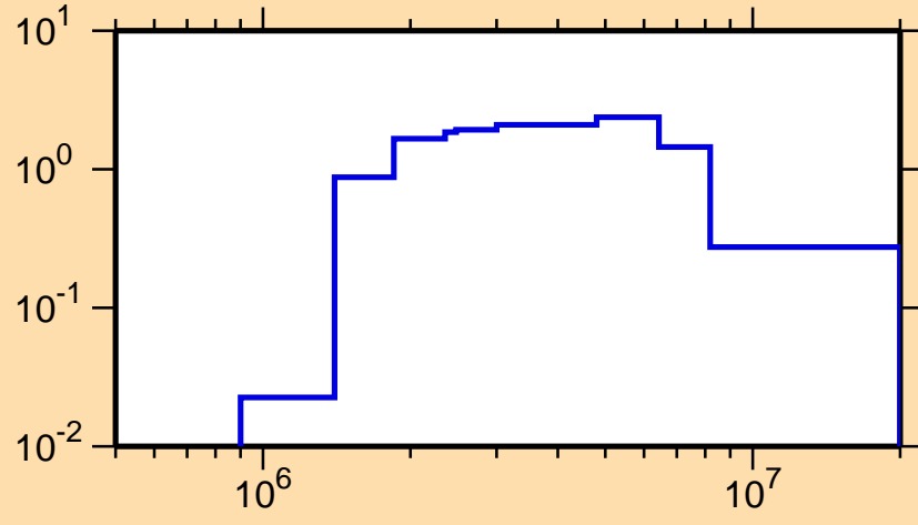
\sigma vs. E for ^{178}\text{Lu}(n,ncont.)
