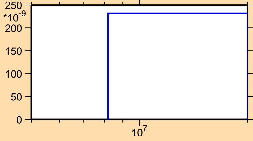
\sigma vs. E for ^{178}\text{Lu}(n,nd)
