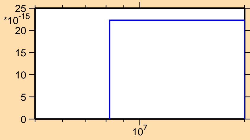
\sigma vs. E for ^{178}\text{Lu}(n,p\alpha)
