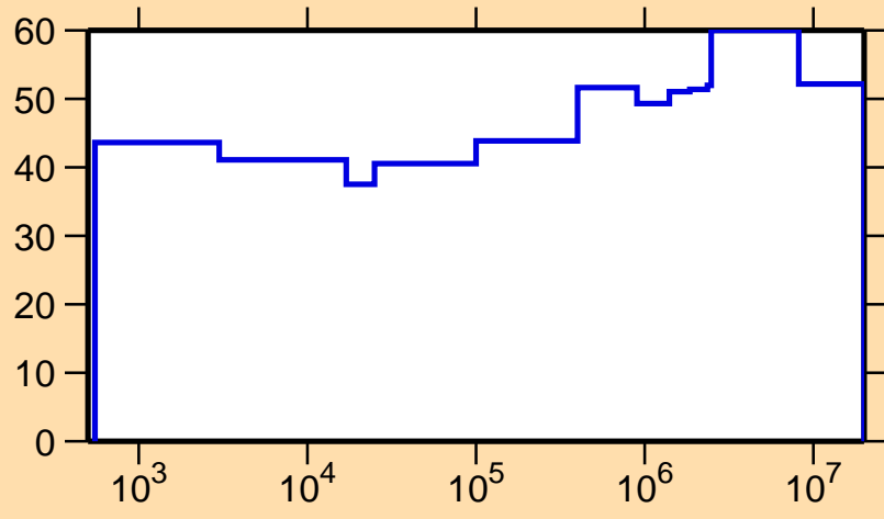
\Delta\sigma/\sigma vs. E for ^{178}\text{Lu}(n,\gamma)
