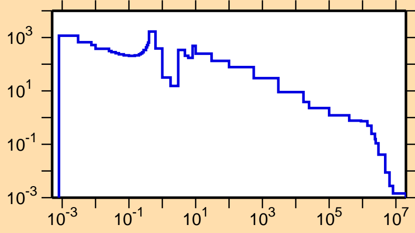
\sigma vs. E for ^{178}\text{Lu}(n,\gamma)
