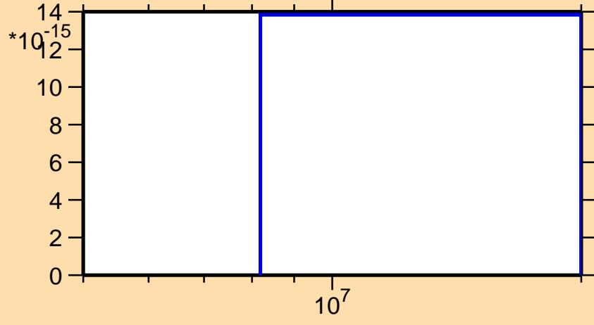
\sigma vs. E for ^{178}\text{Lu}(n,p\alpha)
