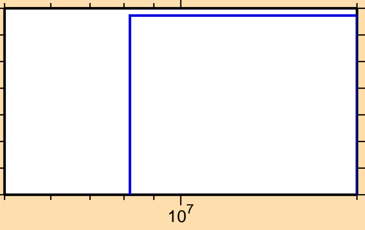
\sigma vs. E for ^{178}\text{Lu}(n,2np)
