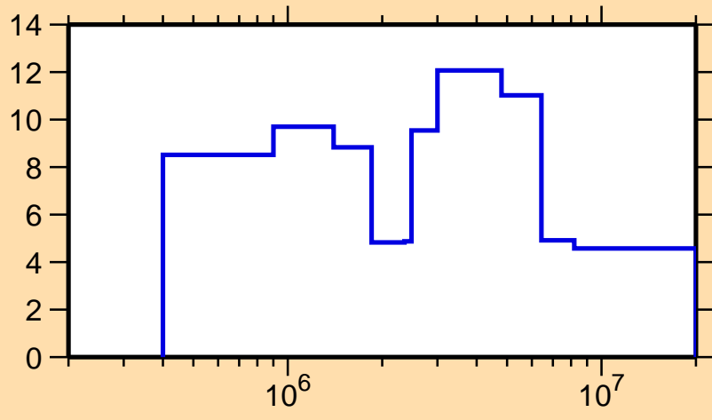
\Delta\sigma/\sigma vs. E for ^{178}\text{Lu}(n, el.)
