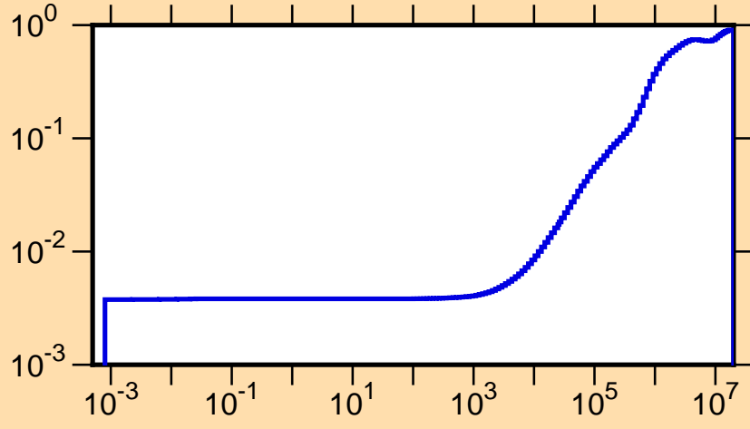
\mu vs. E for ^{179}\text{Lu}(\text{mt251})
