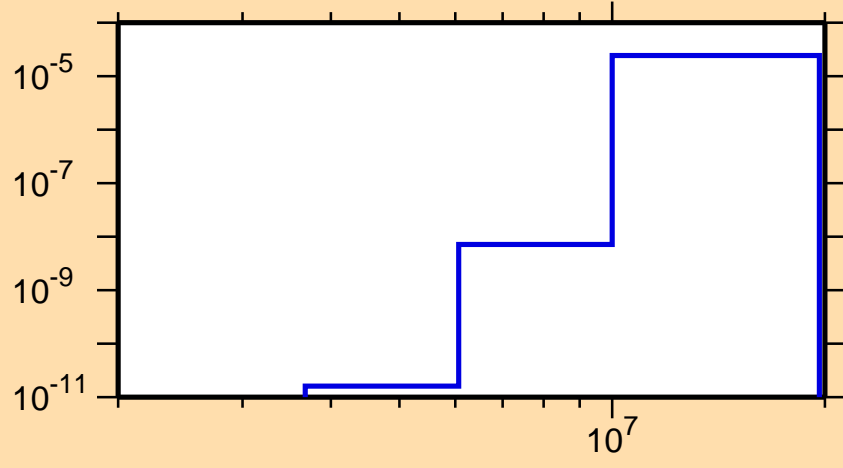
\sigma vs. E for ^{179}\text{Lu}(n,n\alpha)
