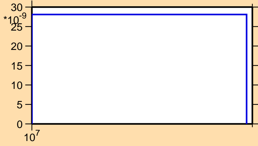
\sigma vs. E for ^{179}\text{Lu}(n,\text{nd})
