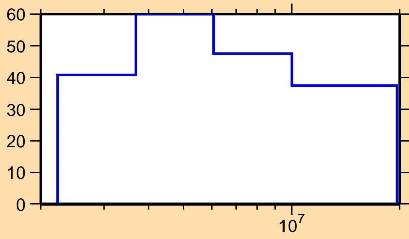
\Delta\sigma/\sigma vs. E for ^{179}\text{Lu}(n,n_1)
