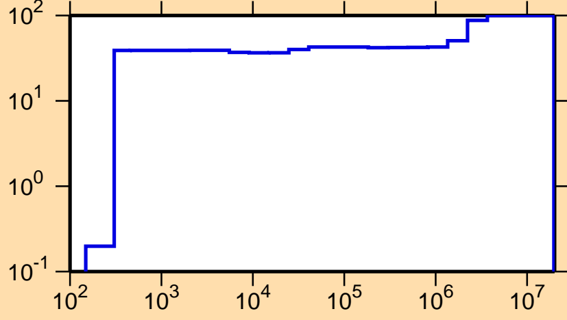
\Delta\sigma/\sigma vs. E for ^{179}\text{Lu}(n,\gamma)
