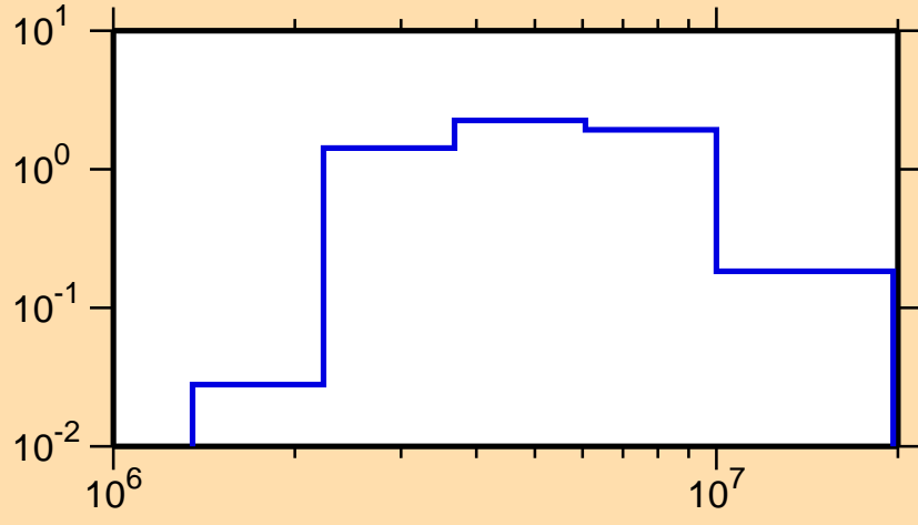
\sigma vs. E for ^{179}\text{Lu}(n,n\text{cont.})
