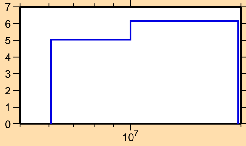
\Delta\sigma/\sigma vs. E for ^{179}\text{Lu}(n,\text{el.})
