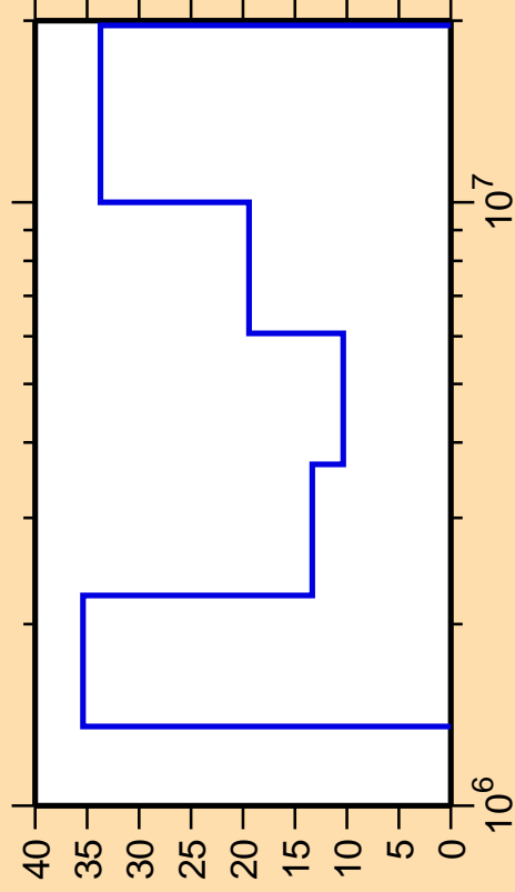
\Delta\sigma/\sigma vs. E for ^{179}\text{Lu}(n,n\text{cont.})
