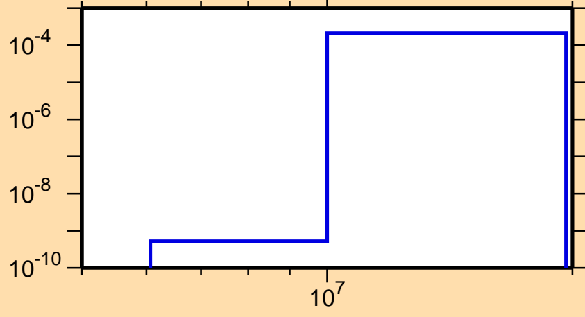
\sigma vs. E for ^{179}\text{Lu}(n,d)
