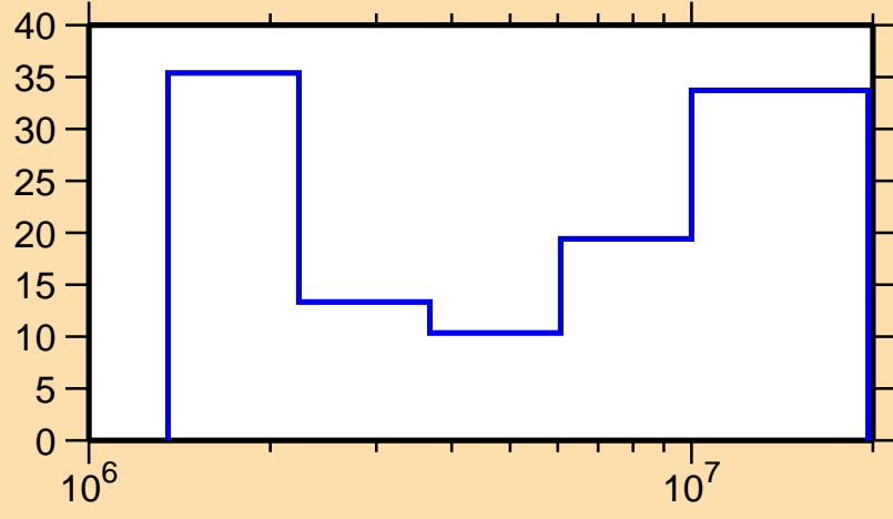
\Delta\sigma/\sigma vs. E for ^{179}\text{Lu}(n,n\text{cont.})
