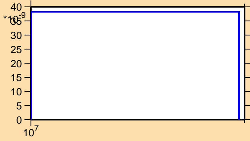
\sigma vs. E for ^{179}\text{Lu}(n,nt)
