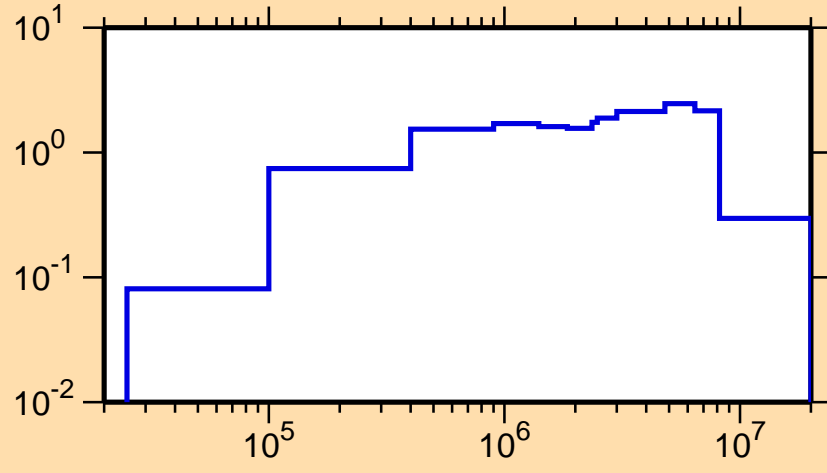
\sigma vs. E for ^{179}\text{Lu}(n,\text{inel.})
