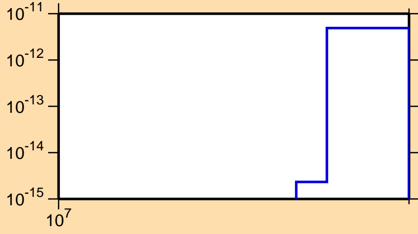
\sigma vs. E for ^{180}\text{Lu}(n,3n\alpha)
