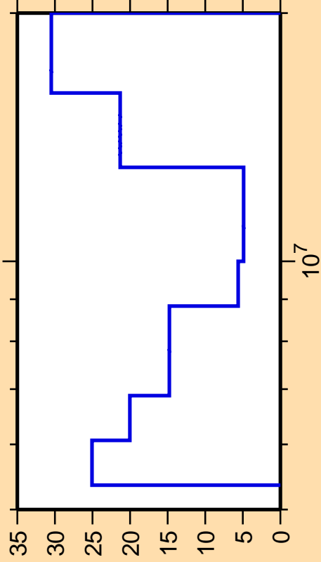
\Delta\sigma/\sigma vs. E for ^{180}\text{Lu}(n,2n)
