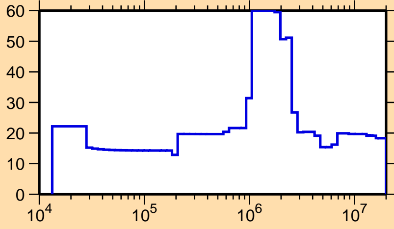
\Delta\sigma/\sigma vs. E for ^{180}\text{Lu}(n,n_1)
