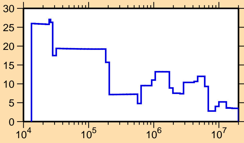
\Delta\sigma/\sigma vs. E for ^{180}\text{Lu}(n,\text{el.})
