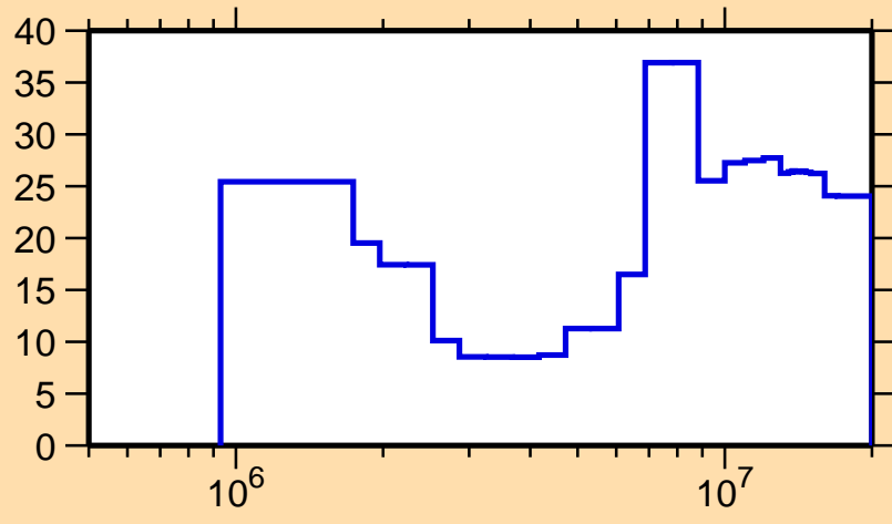
\Delta\sigma/\sigma vs. E for ^{180}\text{Lu}(n,n\text{cont.})
