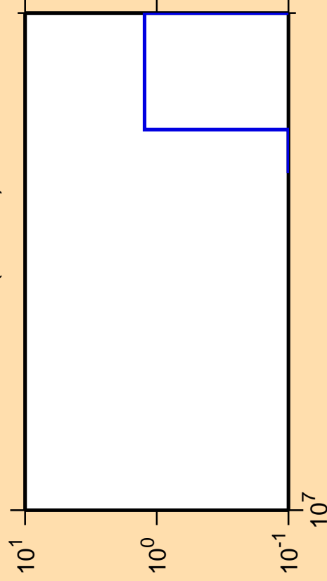
\Delta\sigma/\sigma vs. E for ^{180}\text{Lu}(n,\text{He3})
