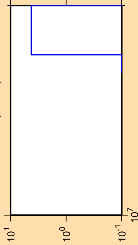
\Delta\sigma/\sigma vs. E for ^{180}\text{Lu}(n,3n\alpha)
