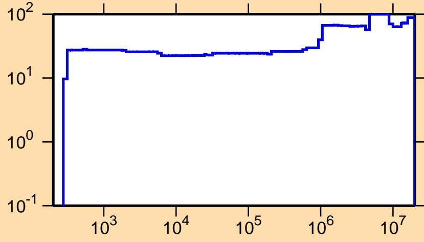
\Delta\sigma/\sigma vs. E for ^{180}\text{Lu}(n,\gamma)
