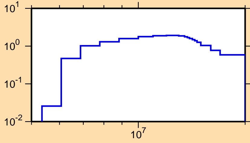
\sigma vs. E for ^{180}\text{Lu}(n,2n)
