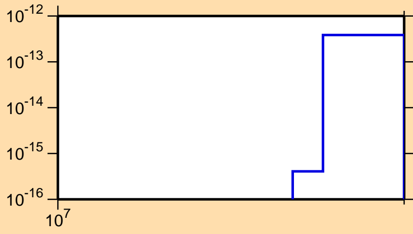
\sigma vs. E for ^{180}\text{Lu}(n,\text{He3})
